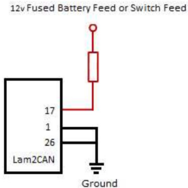
Figure 0-1 – Power and Ground Feeds
