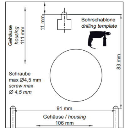
Drilling template on packing
