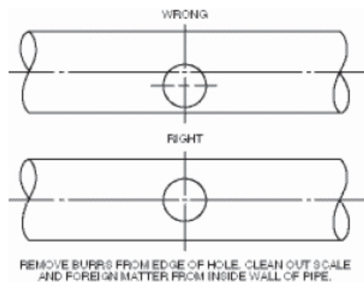
FIGURE 2. MOUNTING HOLE LOCATION:
