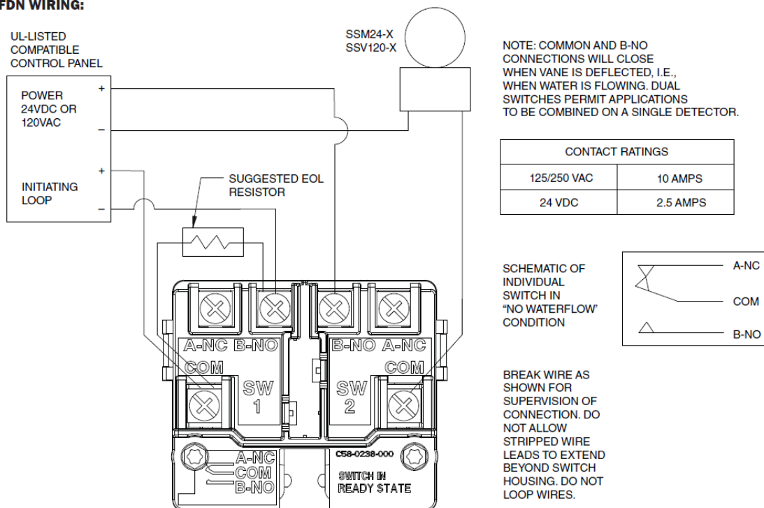
FIGURE 7. WFDN WIRING:
