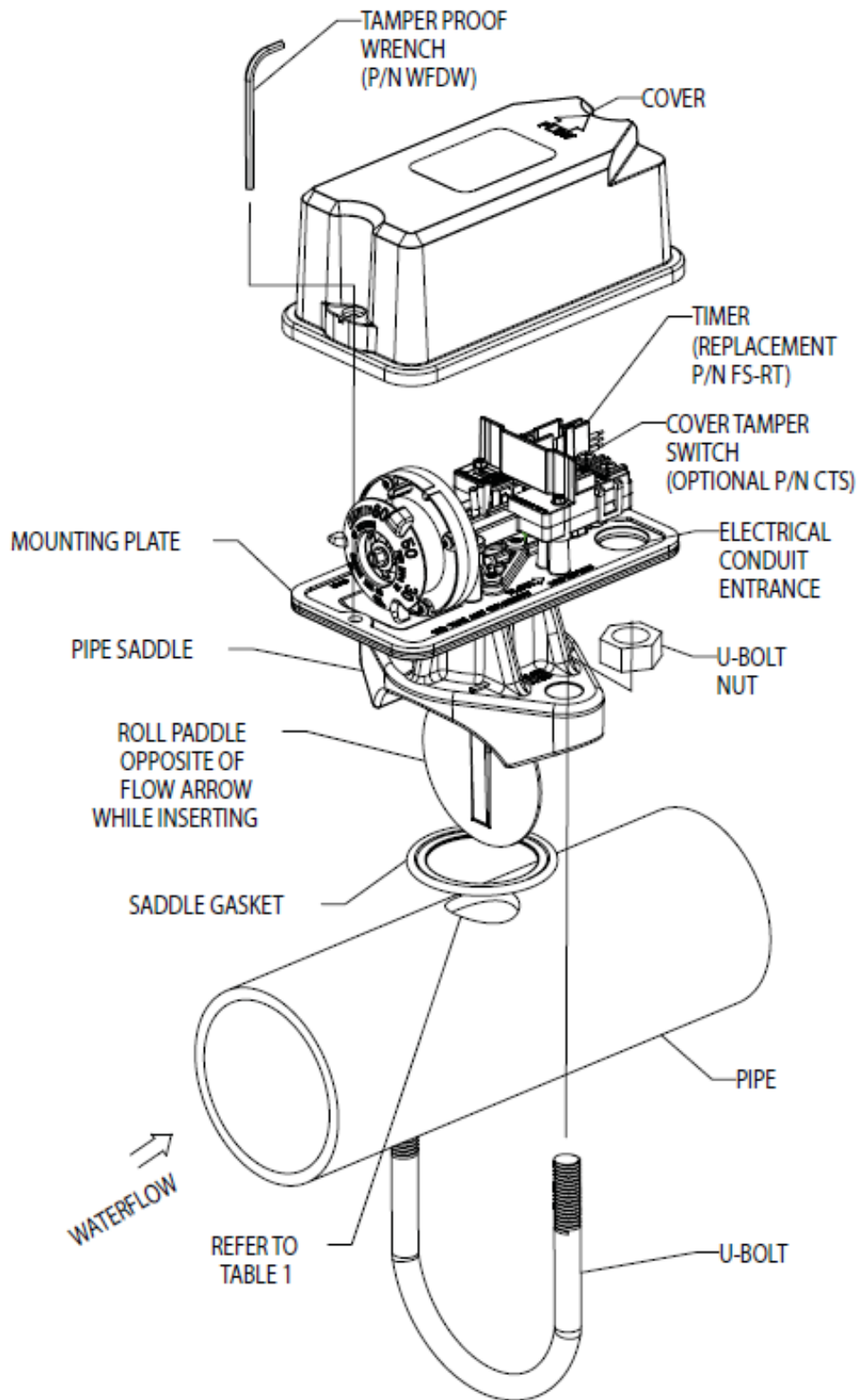
FIGURE 3. ASSEMBLY DIAGRAM:
