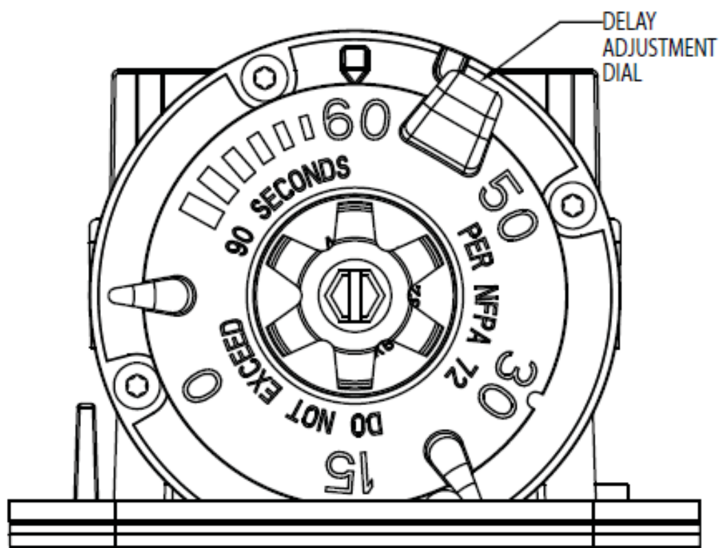
FIGURE 5. DELAY ADJUSTMENT DIAL:
