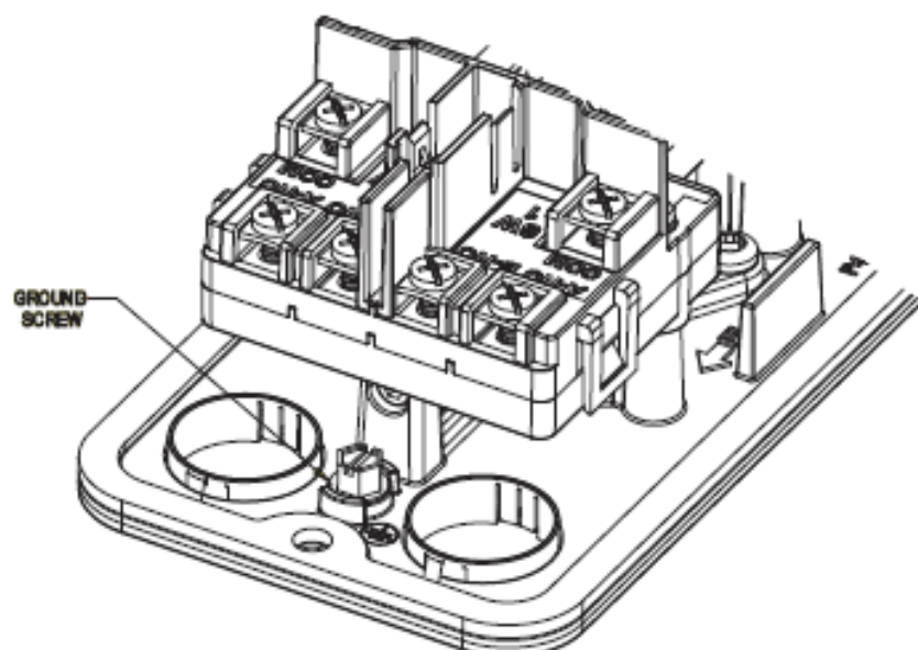
FIGURE 4. KNOCKOUT PLUG REMOVAL:
