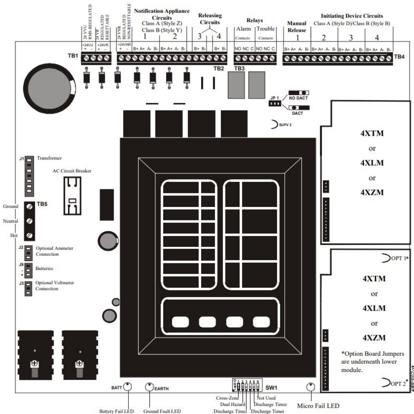
Figure 1 PDRP-1001/PDRP-1001A/PDRP-1001E Installation Diagram
