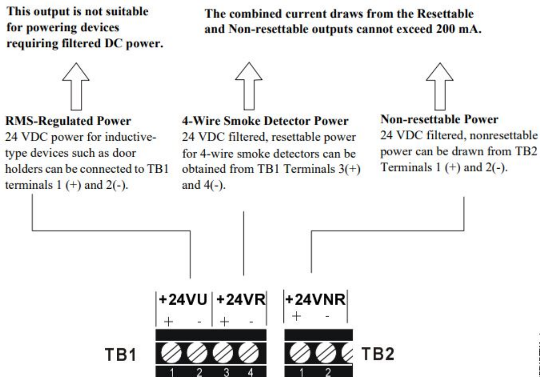
Figure 8 Diagram of Power Terminals
