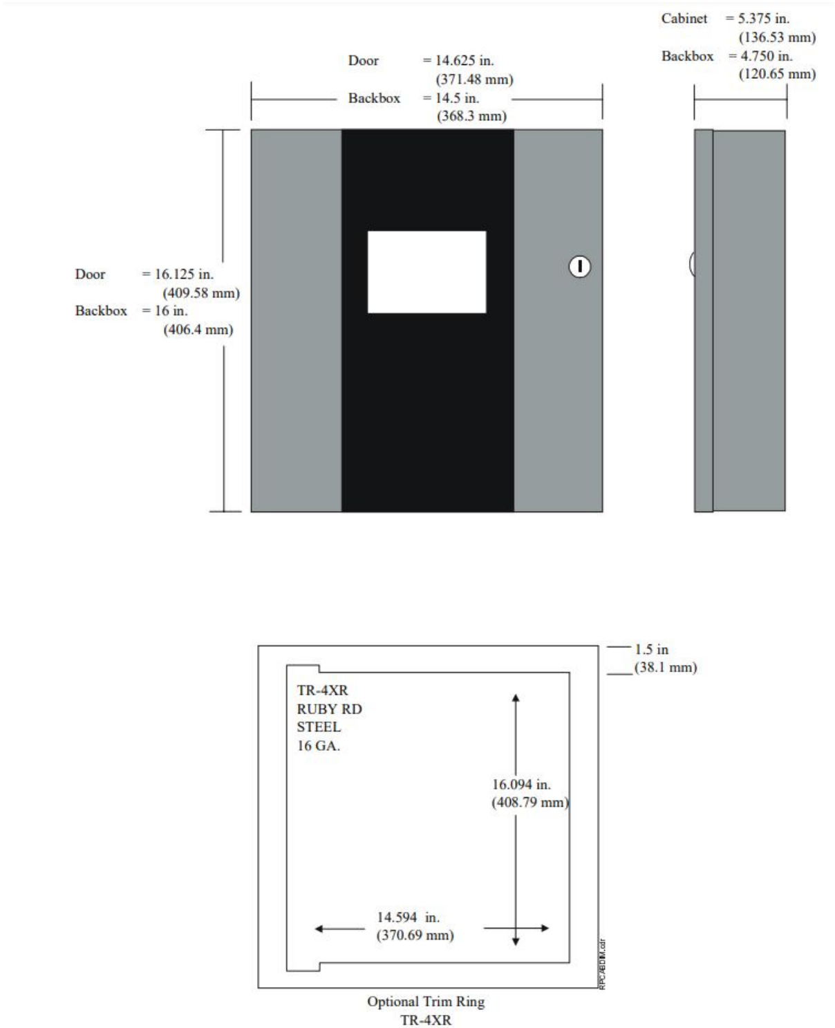
Figure 2 Cabinet Dimensions
