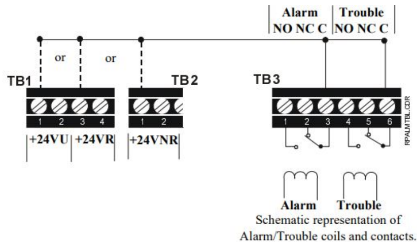
Figure 7 Alarm/Trouble Coils and Contacts
