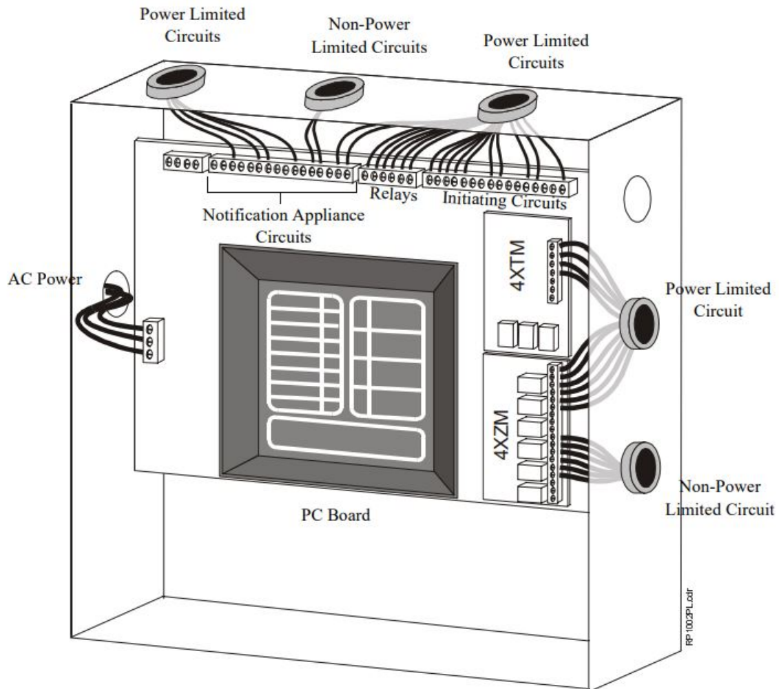
Figure 3 Typical Wiring Diagram for UL Power Limited Requirements
