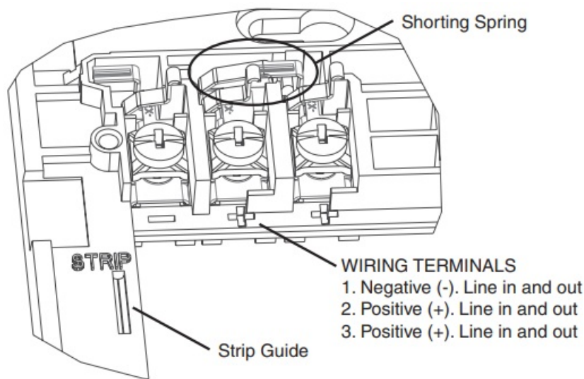
FIGURE 5. WIRING TERMINALS, SHORTING SPRING, AND STRIP GUIDE
