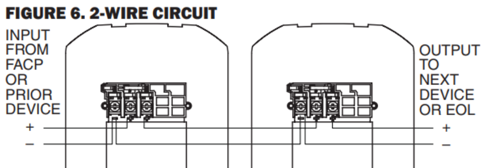
FIGURE 6. 2-WIRE CIRCUIT
