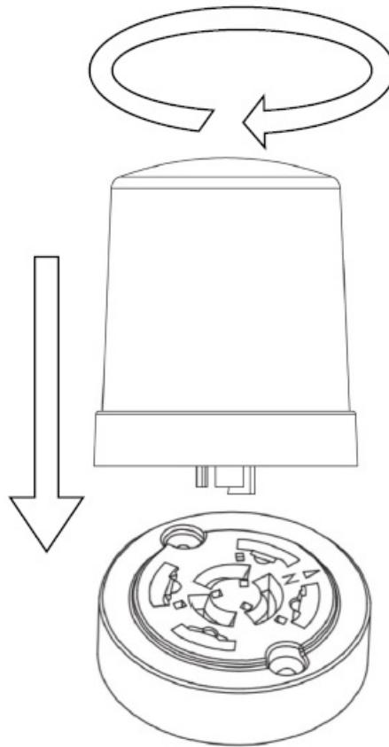
Figure 2 – Installation Diagram
