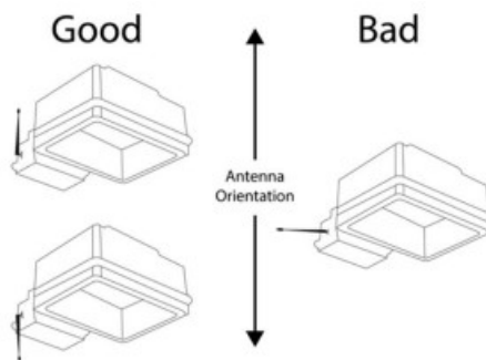
Figure 1 - Proper External Antenna Installation
