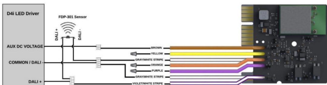
Figure 2 – D4i Wiring Diagram
