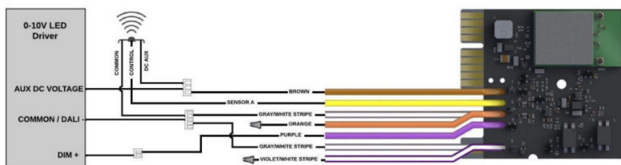
Figure 1 - DIM to OFF Wiring Diagram
