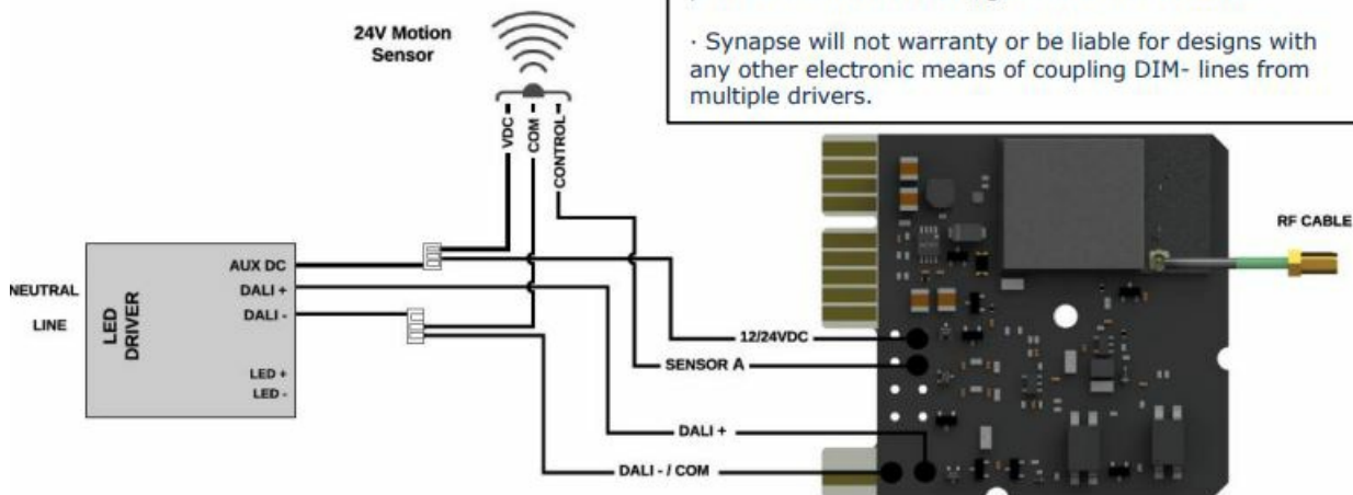
Figure 3 – D4i Wiring Diagram
