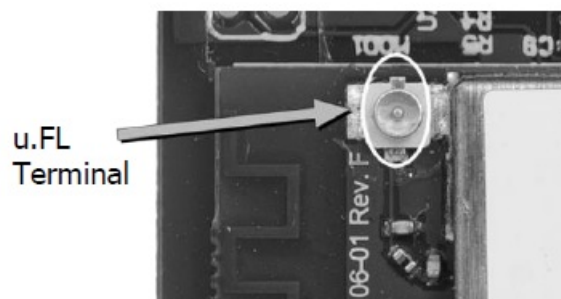
Figure 4- u.FL Terminal
