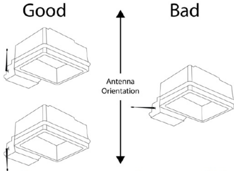
Figure 1 - Proper External Antenna Installation
