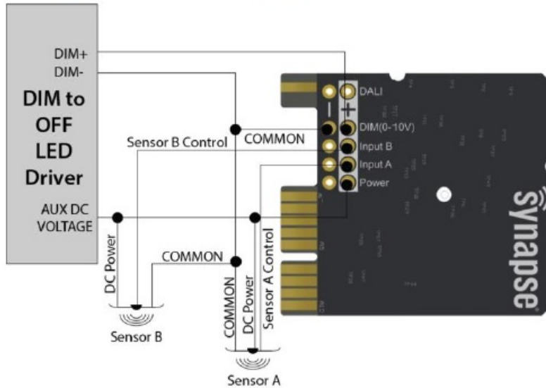
Figure 2 – Dim to OFF Wiring Diagram
