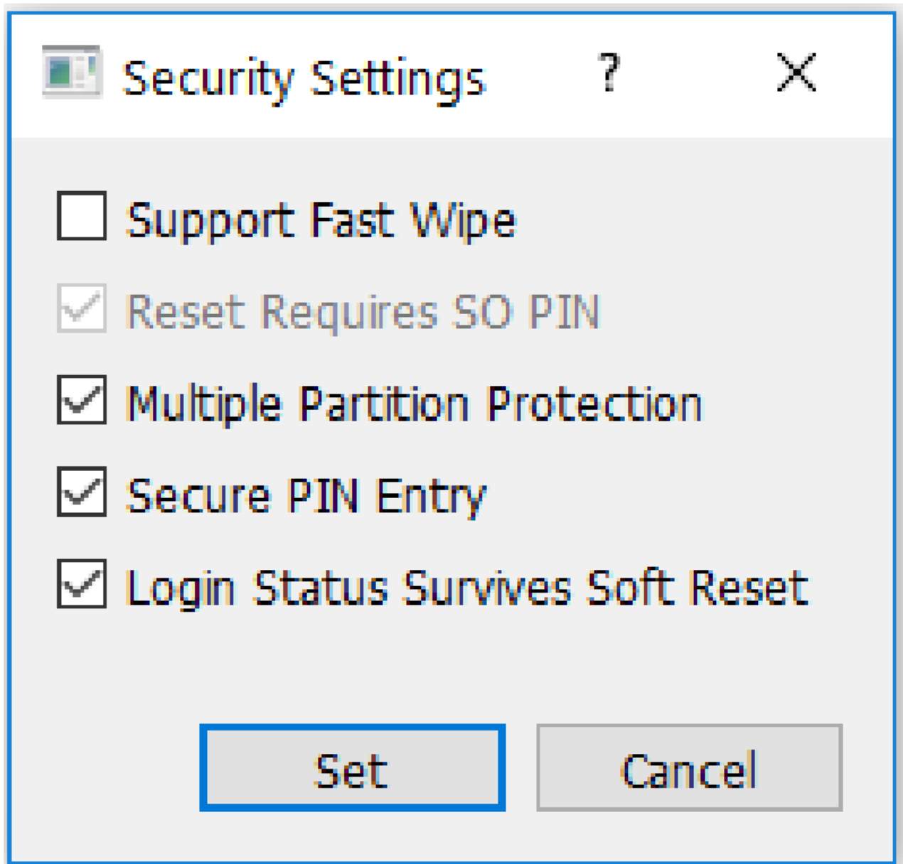
Fig. 1 Security Settings
