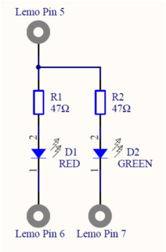
Figure 8: Tally circuit
