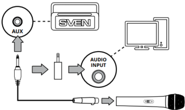
Fig. 1. Connection diagram/Puc.
