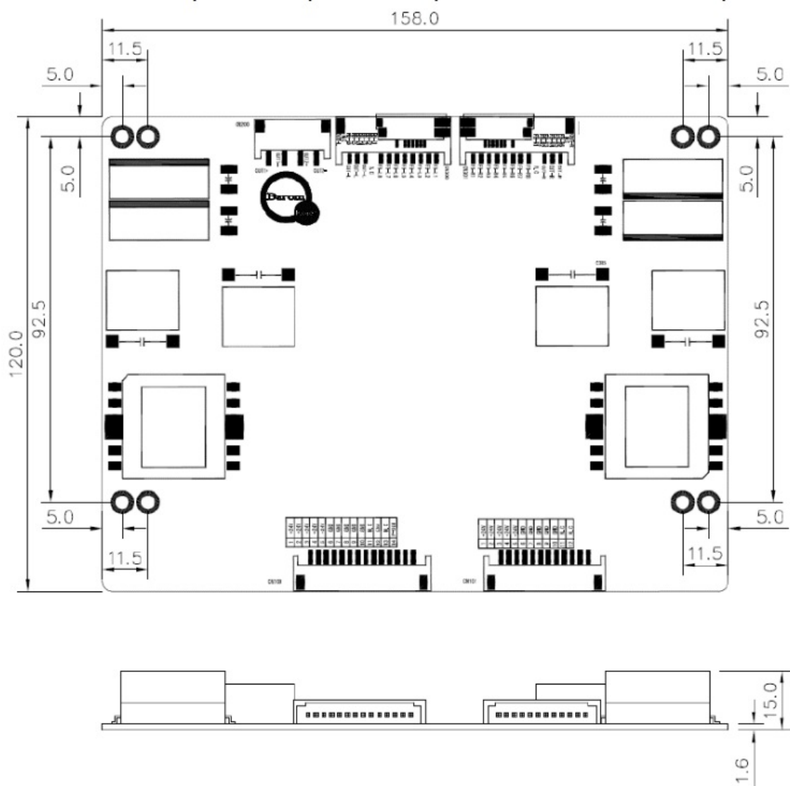
LED Driver Board (GP-1520LD) Dimension (158.0mm x 120mm x 15.0mm)
