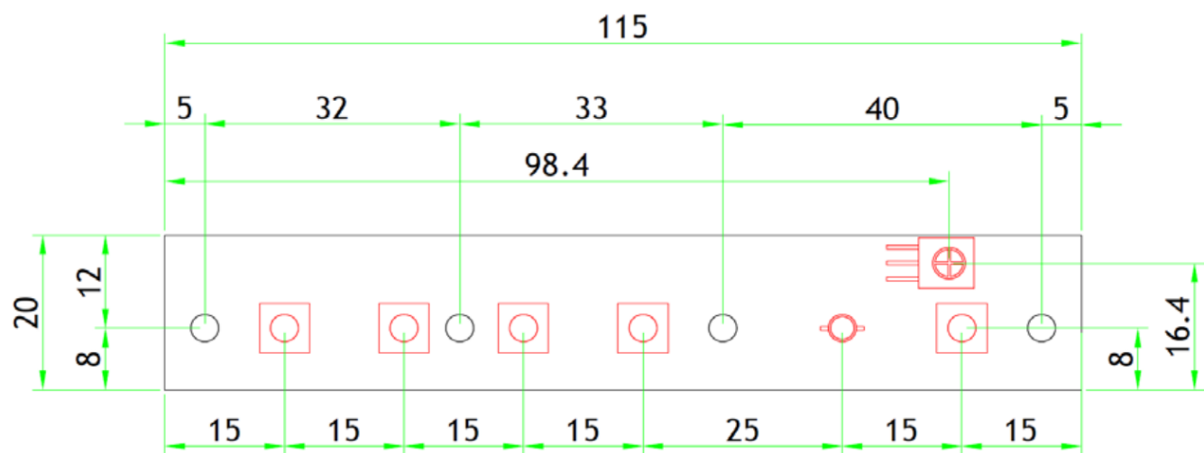
OSD Board (K002) Dimension (115mm x 20mm x 8.7mm)
