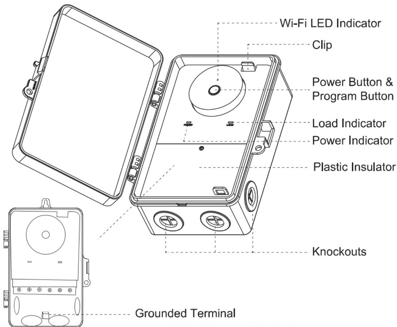
FIG.1 Product Illustration
