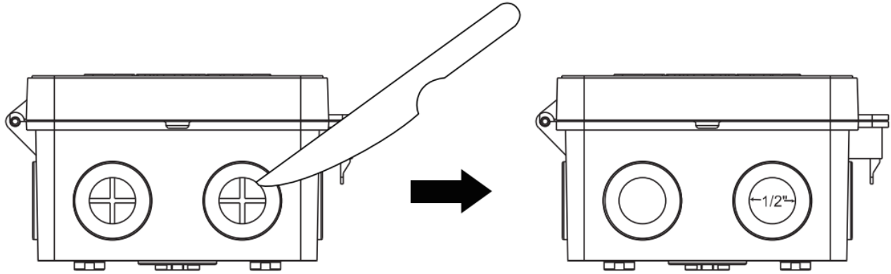
FIG.2 1/2" knockout
