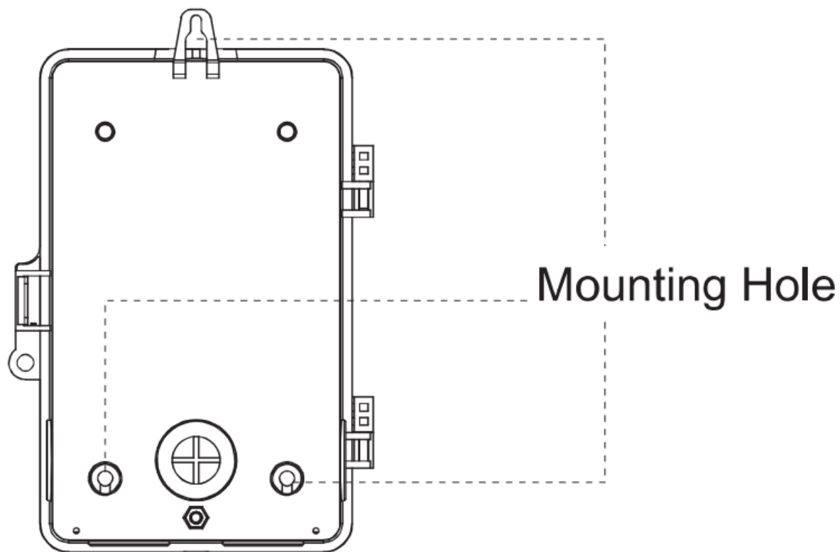
FIG.4 Mounting Holes
