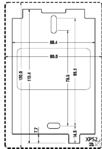
Drilling Template
