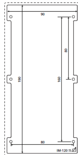
Drilling Template
