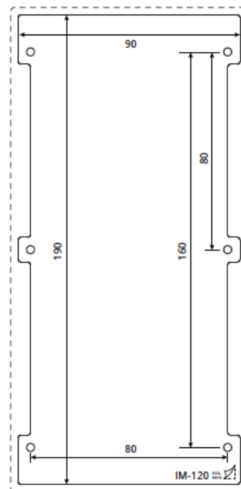
Drilling Template
