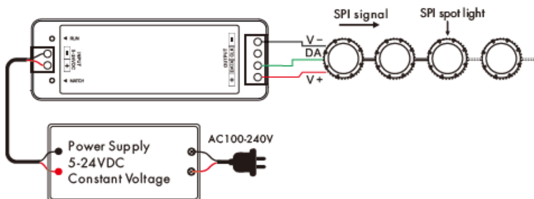
SC connect with SPI pixel strip (LPD6803)
