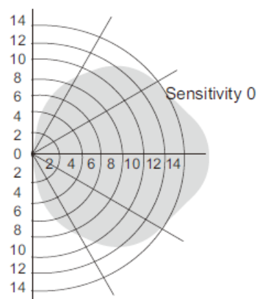
Wall Pattern (Unit: m) Installation Height: 10m
