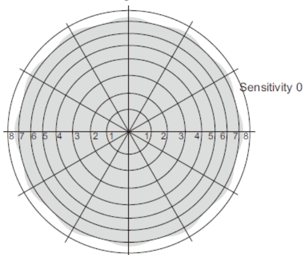
Ceiling Pattern (Unit: m) Installation Height: 5m
