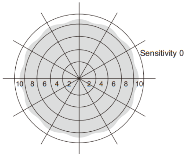
Ceiling Pattern (Unit: m) Installation Height: 2.5m
