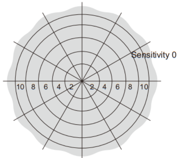
Ceiling Pattern (Unit: m) Installation Height: 10m
