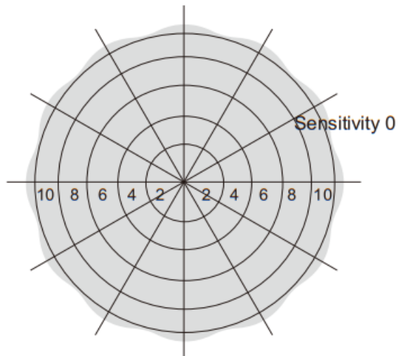
Ceiling Pattern (Unit: m) Installation Height: 5m
