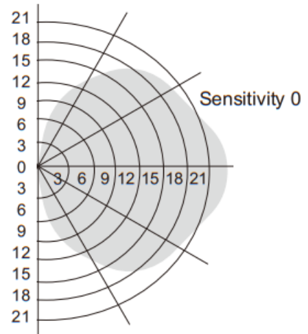
Wall Pattern (Unit: m) Installation Height: 2.5m
