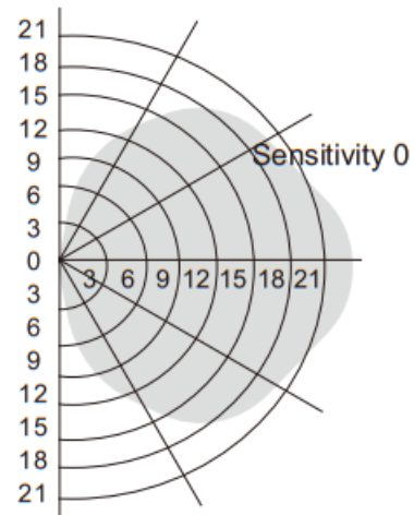
Wall Pattern (Unit: m) Installation Height: 5m
