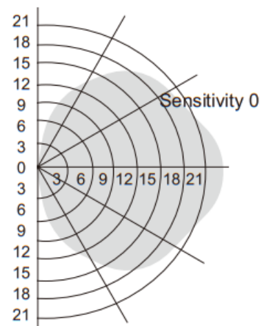
Wall Pattern (Unit: m) Installation Height: 10m
