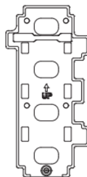
Button Membrane (4-Button shown)
