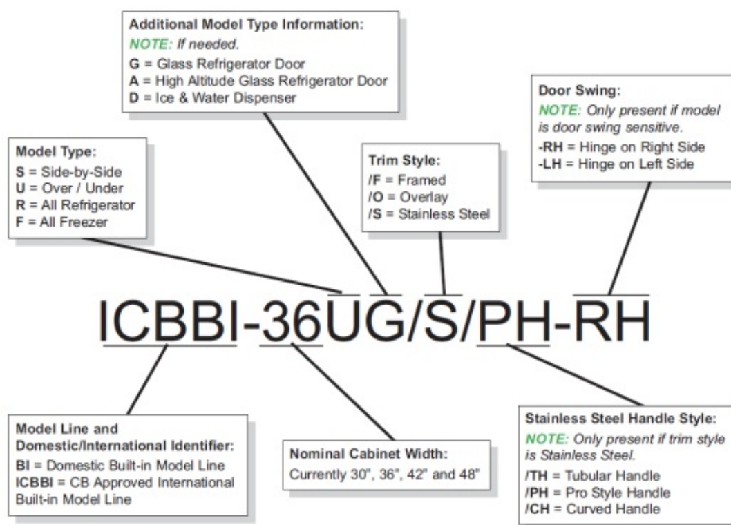
Figure 1-2. Model Number Code
