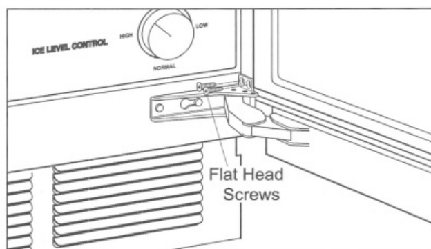
Figure 2-4. Securing Unit to Cabinet
