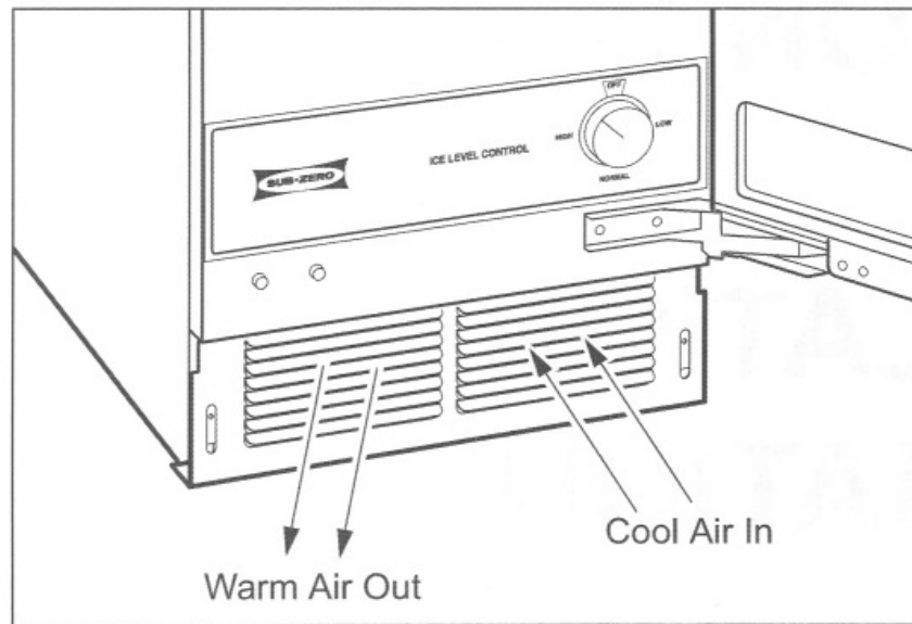
Figure 2-1. Condenser Air Flow
