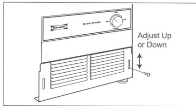
Figure 2-6. Kickplate/Grille Adjustment
