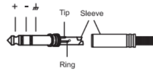
1/4" TRS jack Balanced input/output
