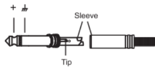
1/4" TS jack Unbalanced input/output
