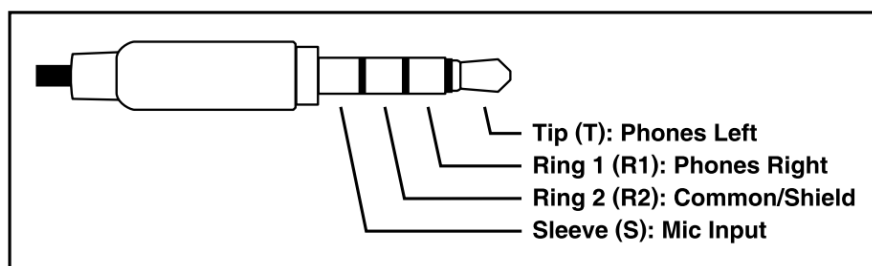
Figure 3. Headset B connection pinout chart
