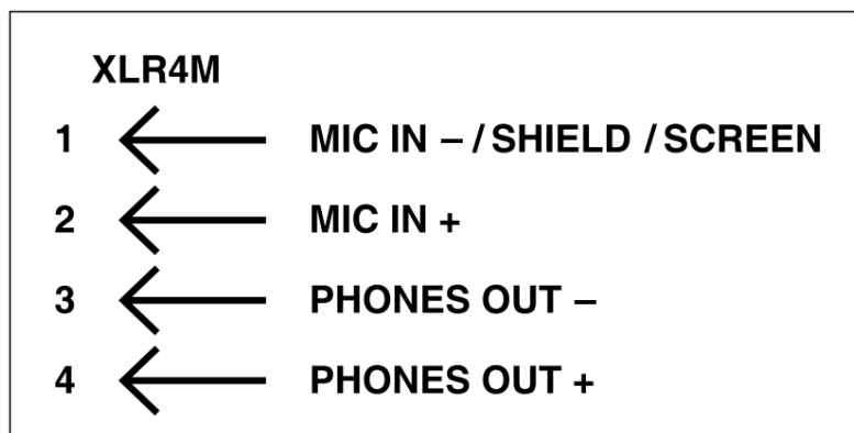
Figure 2. Headset A connection pinout chart
