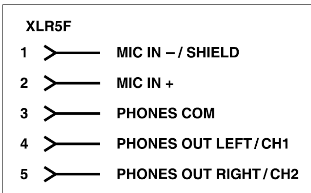
Figure 2. Headset connection pinout chart
