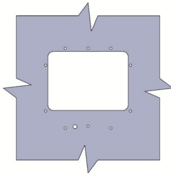
Panel Cutout 120mm x 140mm
