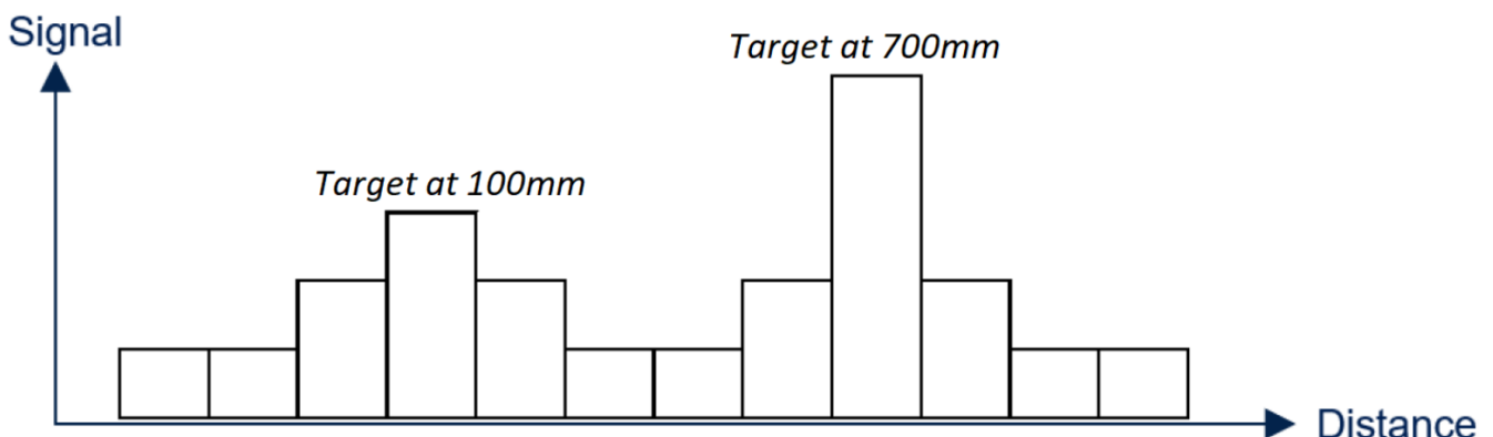
Figure 11. Example of histogram with two targets
