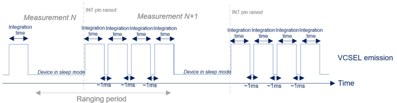
Figure 9. Integration time for 8×8 autonomous
