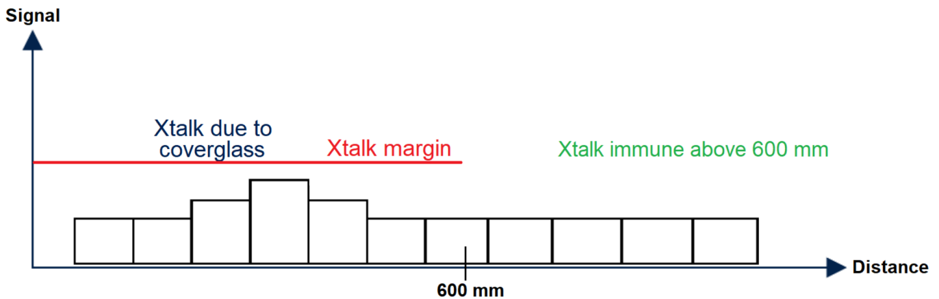
Figure 12. Xtalk margin
