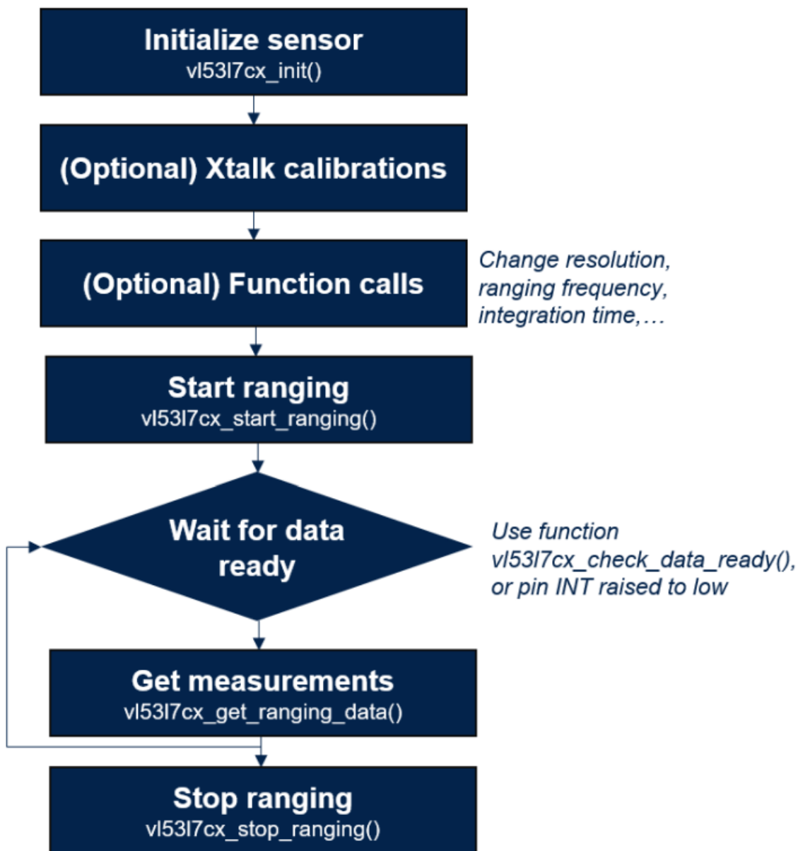
Figure 7. Ranging flow using VL53L7CX
