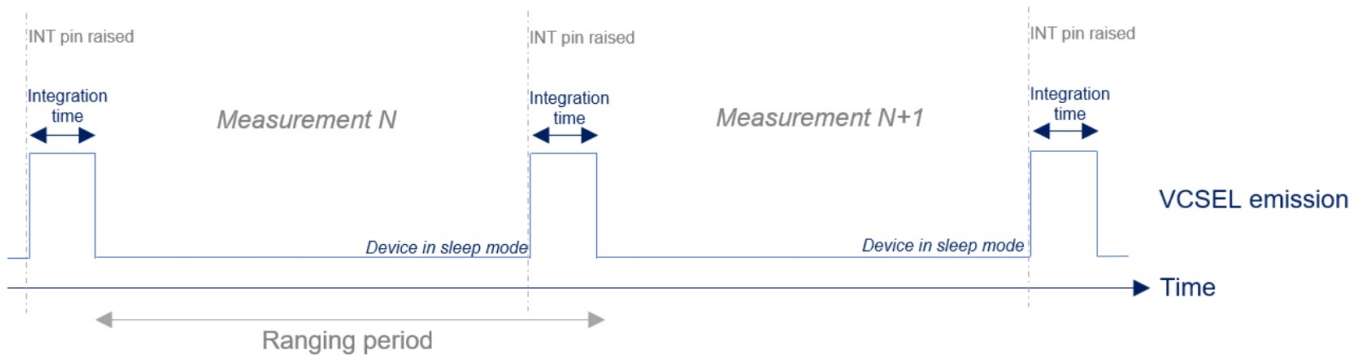
Figure 8. Integration time for 4×4 autonomous
