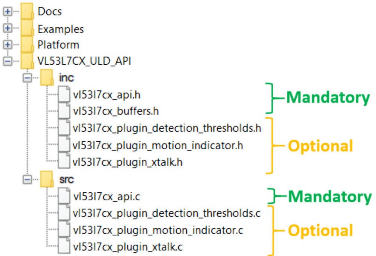
Figure 5. Driver architecture
