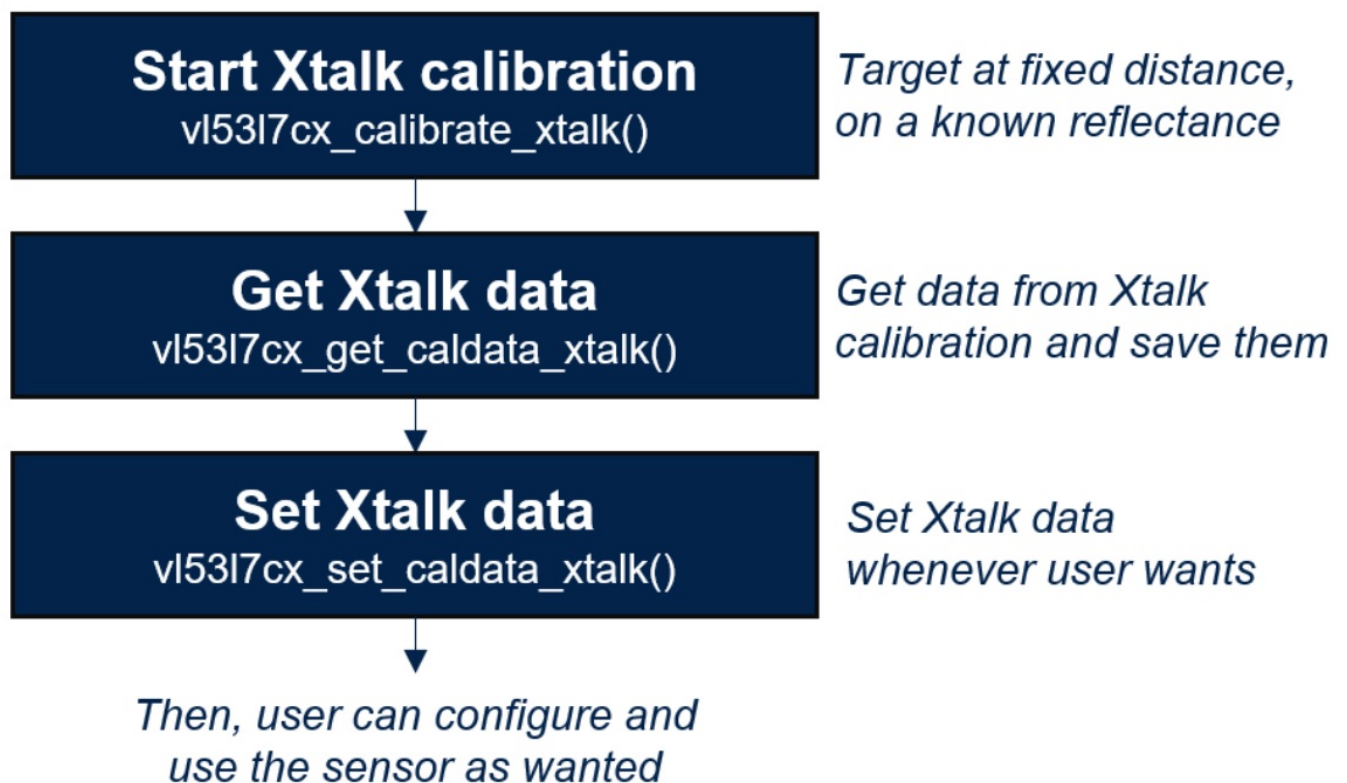
Figure 6. Crosstalk calibration flow
