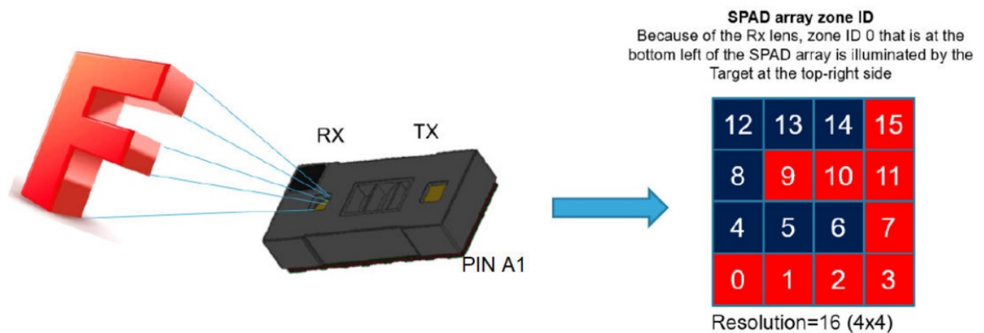
Figure 3. VL53L5CX effective orientation
