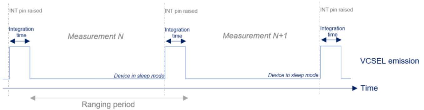
Figure 8. Integration time for 4x4 autonomous
