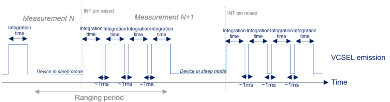
Figure 9. Integration time for 8x8 autonomous
