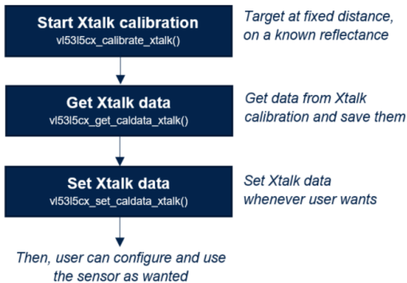
Figure 6. Crosstalk calibration flow
