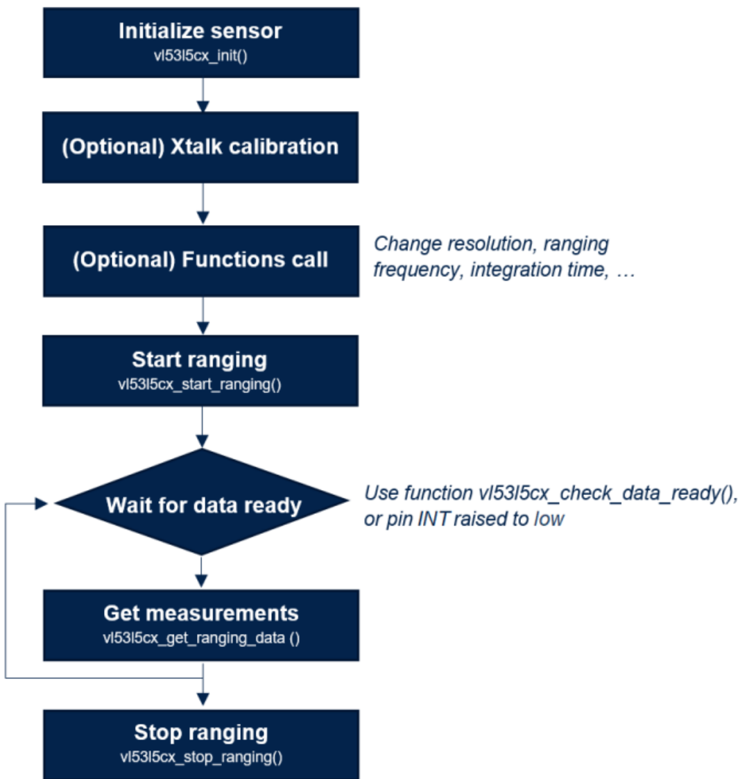
Figure 7. Ranging flow using VL53L5CX
