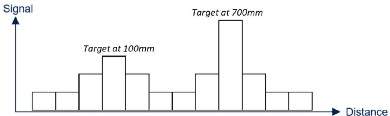
Figure 11. Example of histogram with two targets
