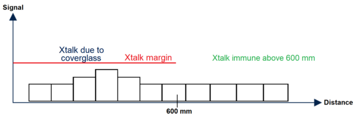
Figure 12. Xtalk margin
