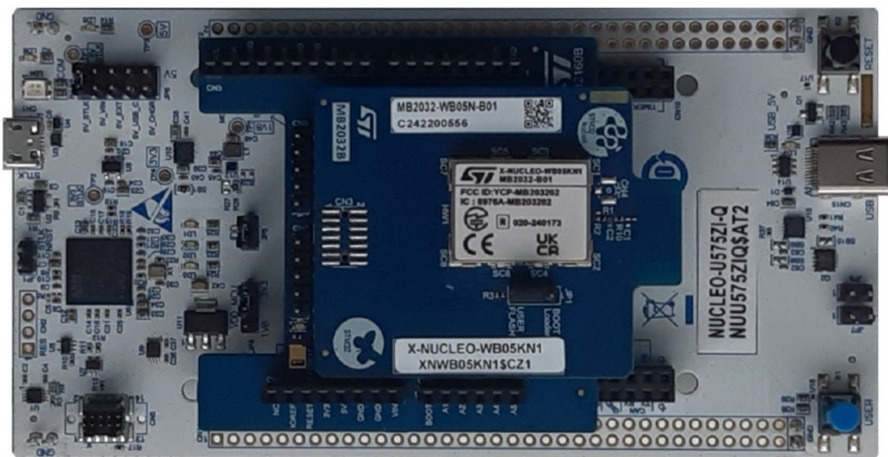
Figure 2. X-NUCLEO-WB05KN1 plugged into NUCLEO-U575ZI-Q
