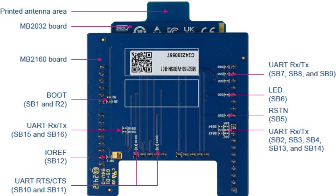
Figure 4. X-NUCLEO-WB05KN1 PCB bottom view
