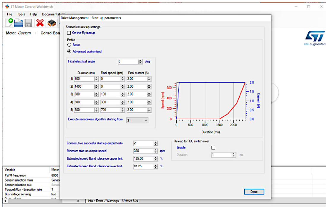
Figure 8. X-CUBE-MCSDK configuration example (2 of 2)
