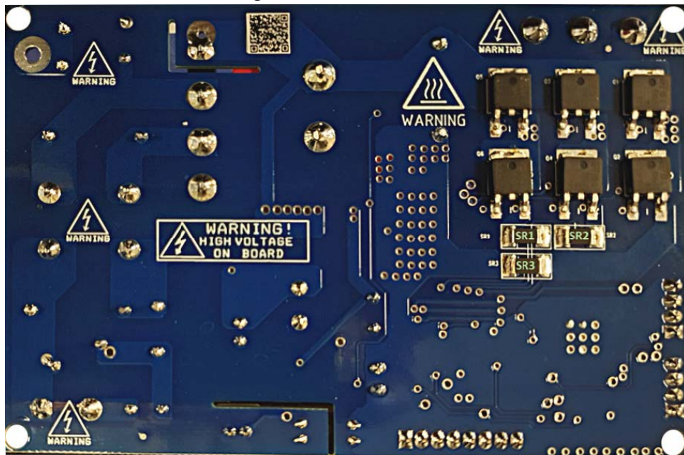
Figure 4. STEVAL-CTM012V1 – shunt configuration
