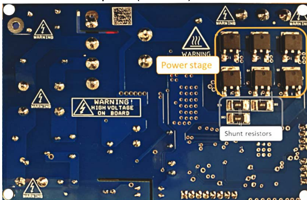
Figure 3. STEVAL-CTM012V1 main components (bottom view)
