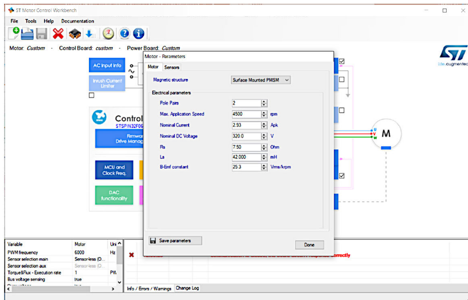
Figure 8. X-CUBE-MCSDK configuration example (2 of 2)
