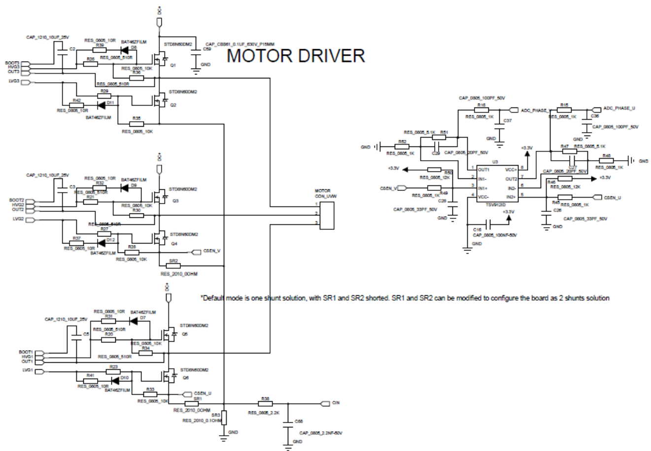
Figure 13. STEVAL-CTM012V1 circuit schematic (2 of 2)
