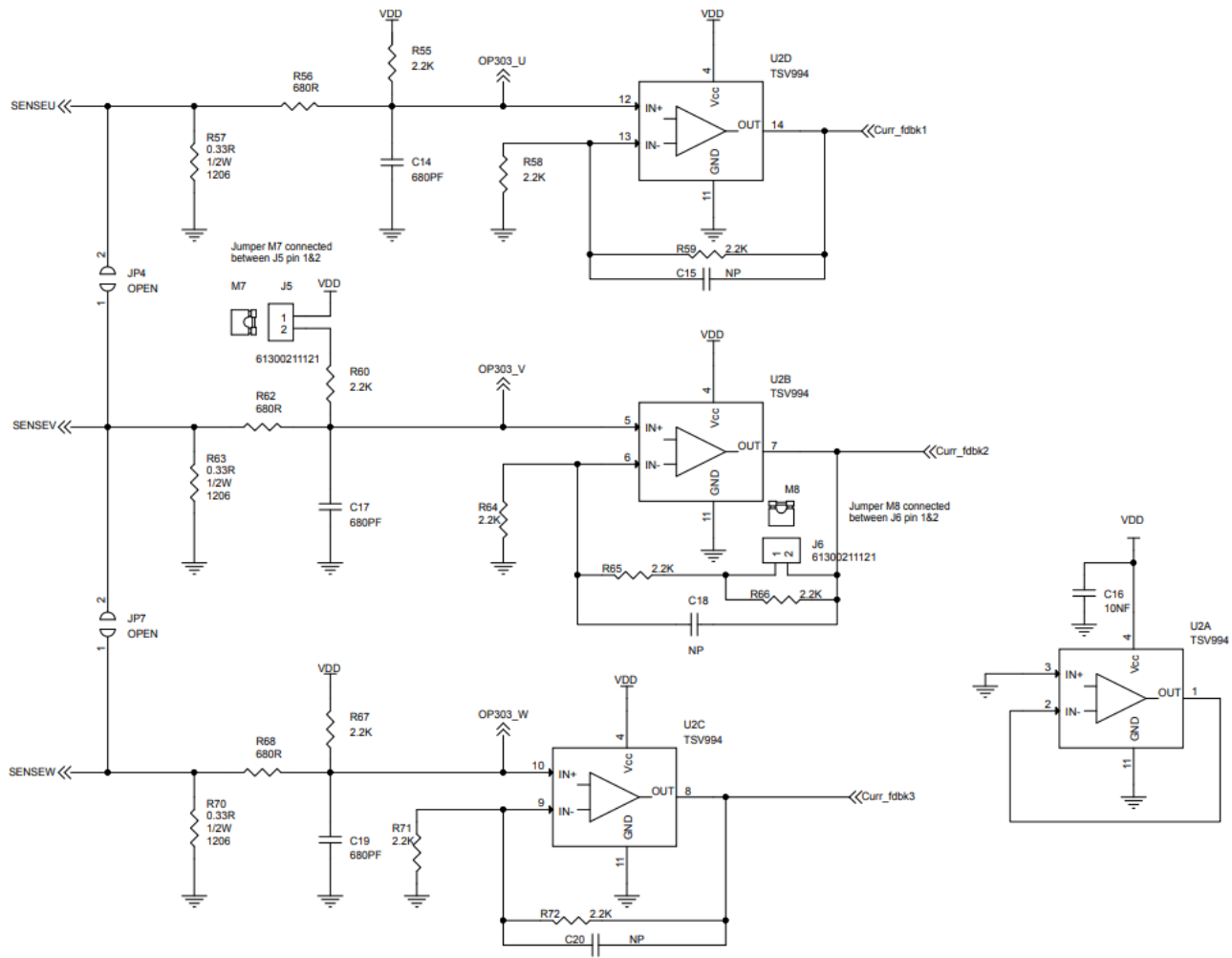
Figure 8. X-NUCLEO-IHM16M1 circuit schematic (5 of 5)
