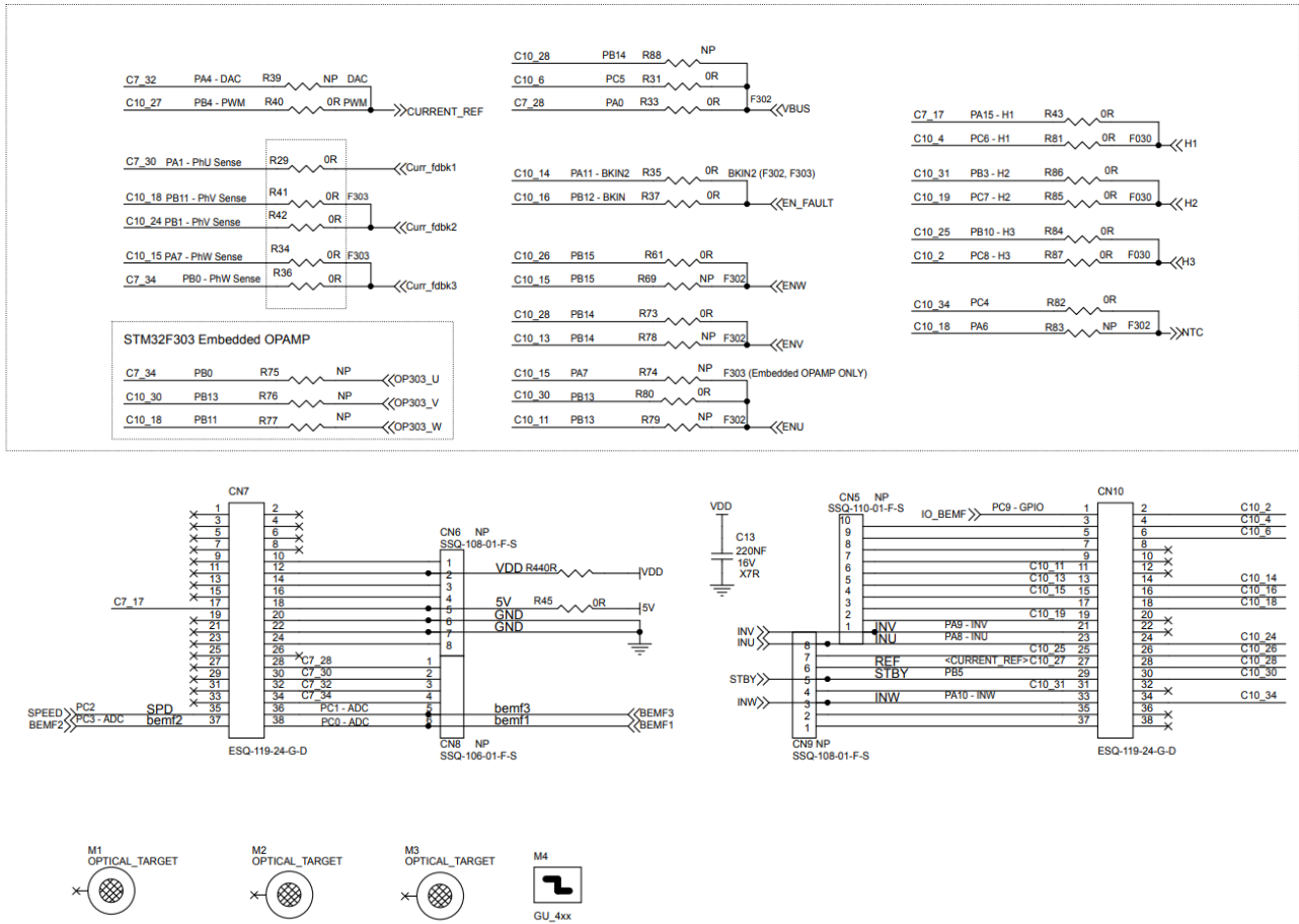
Figure 6. X-NUCLEO-IHM16M1 circuit schematic (3 of 5)
