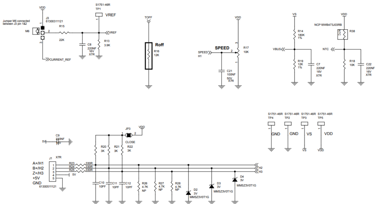
Figure 5. X-NUCLEO-IHM16M1 circuit schematic (2 of 5)
