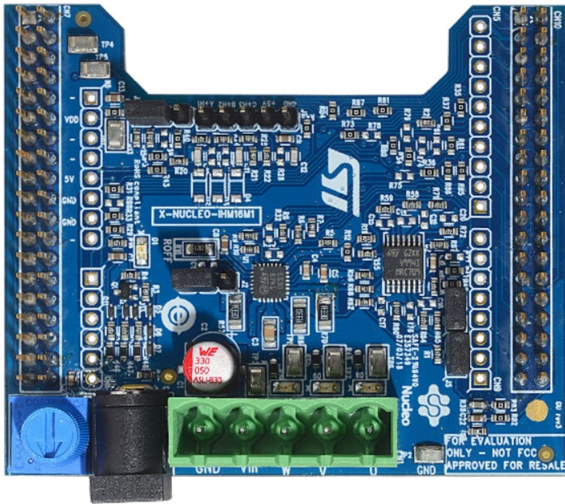
Figure 1. X-NUCLEO-IHM16M1 expansion board
