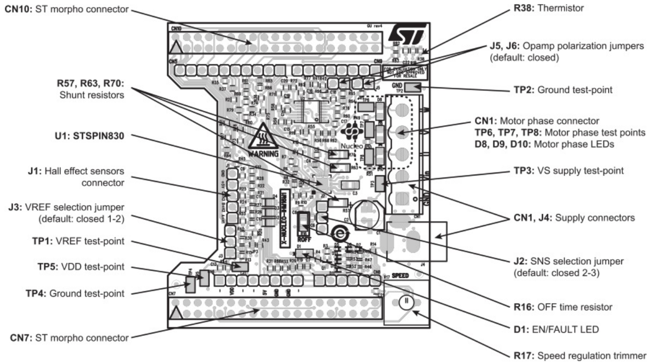
Figure 2. X-NUCLEOIHM16M1 component positions
