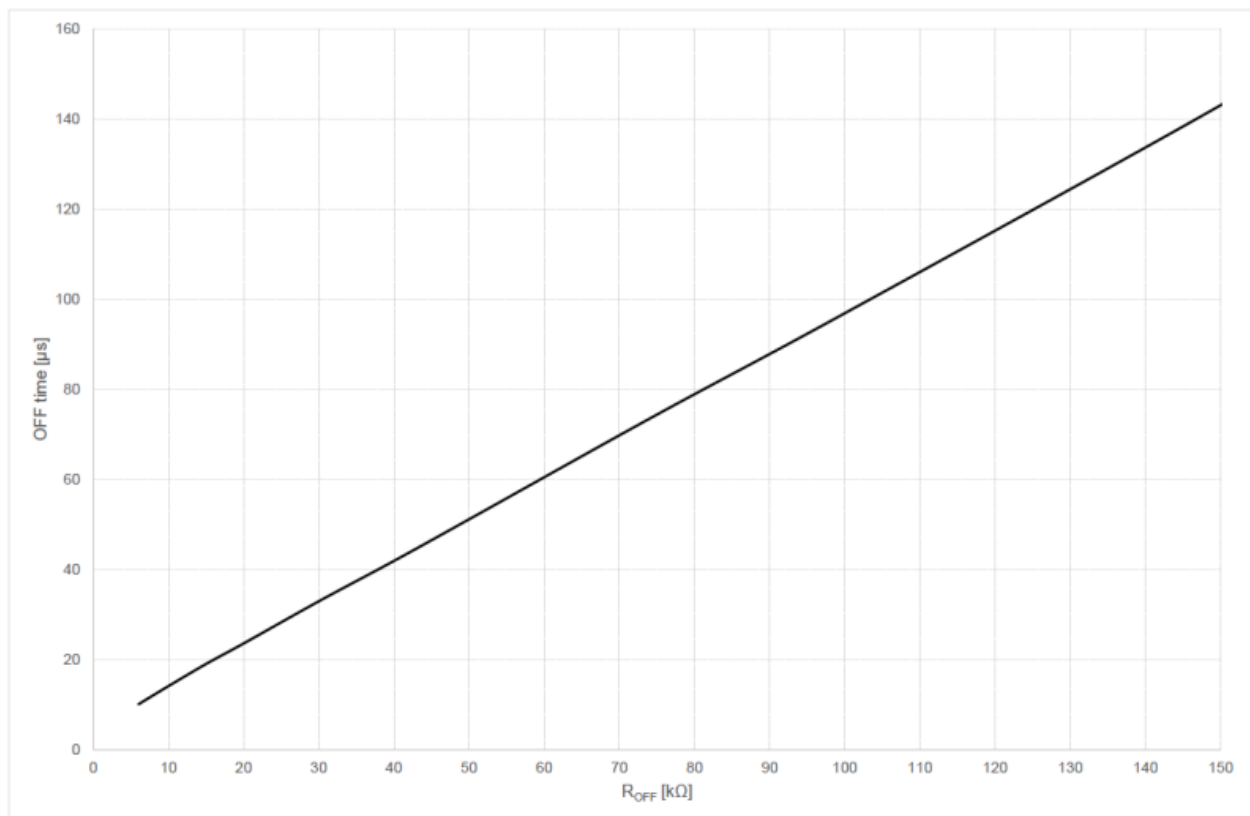
Figure 3. OFF time vs. R_{OFF} value
