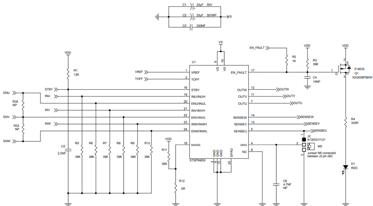
Figure 4. X-NUCLEO-IHM16M1 circuit schematic (1 of 5)
