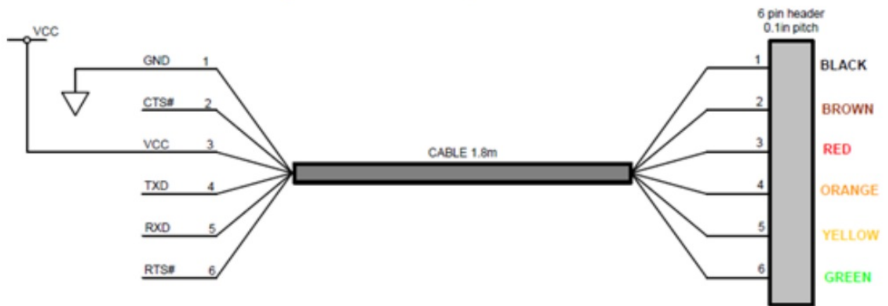
Figure 5. STNRG328S pin connections
