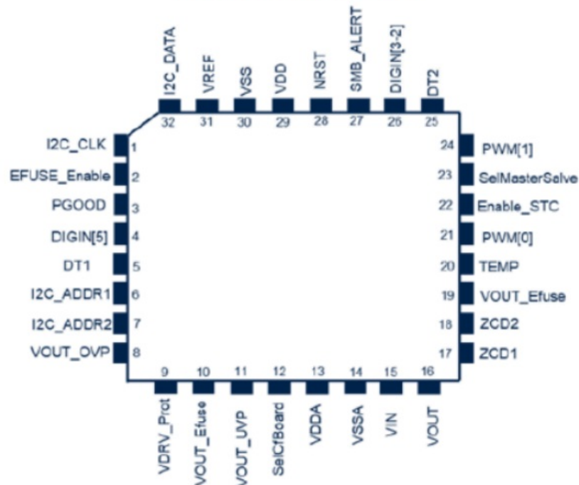
Figure 4. STNRG328S pinout
