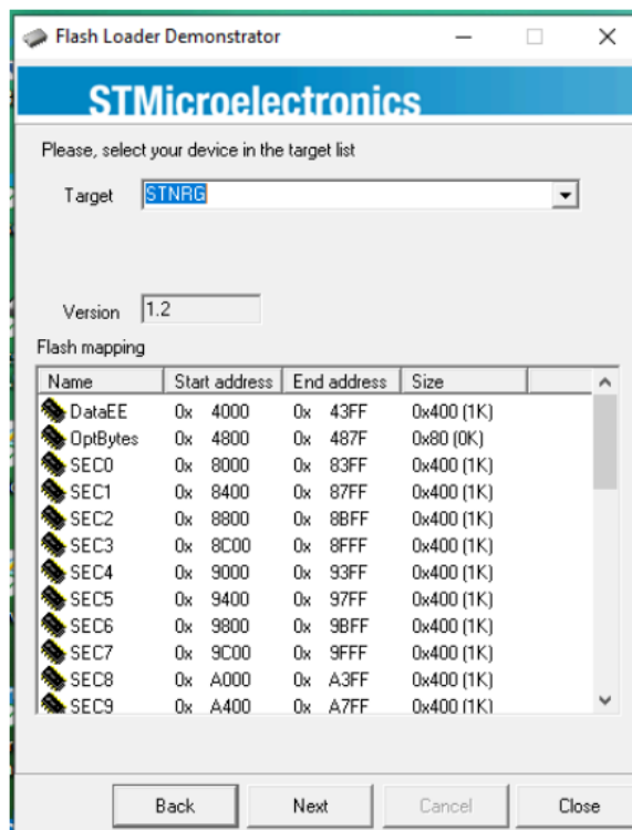
Figure 8. ST Flash Loader – STNRG NVM map
