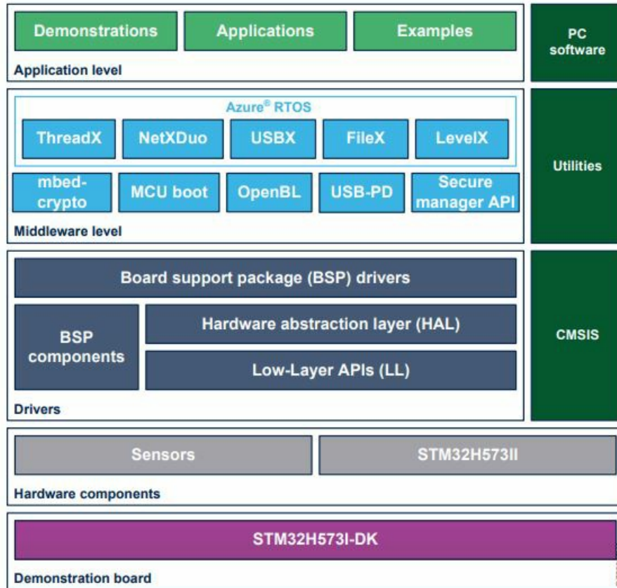
Figure 1. STM32CubeH5 MCU Package architecture
