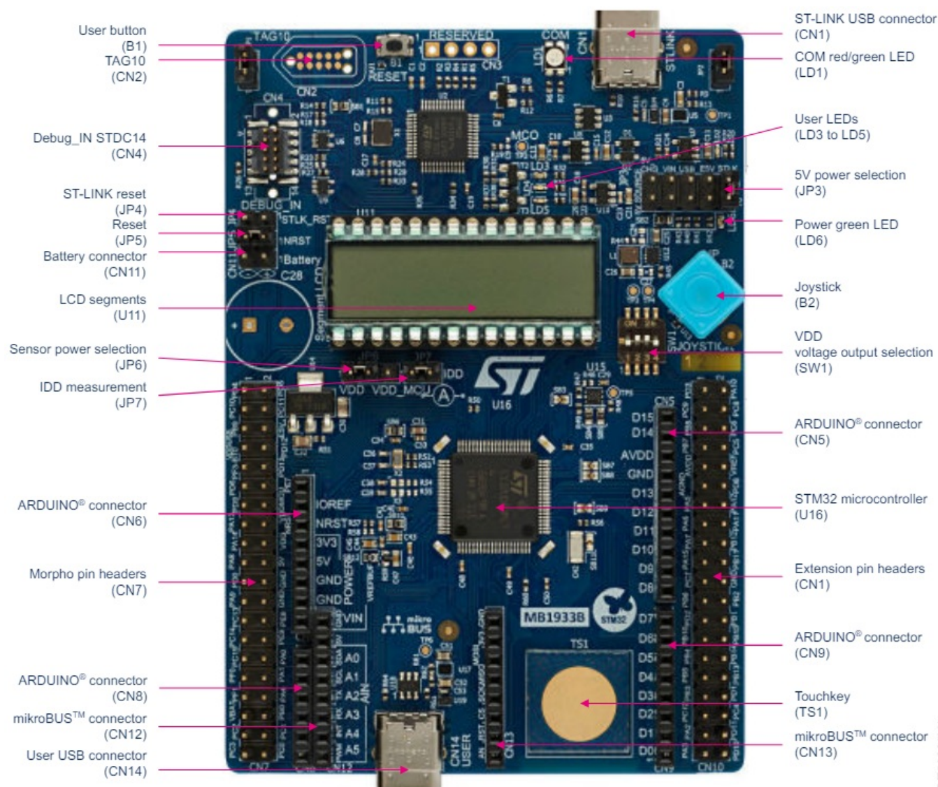
Figure 2. STM32U083C-DK Discovery board
