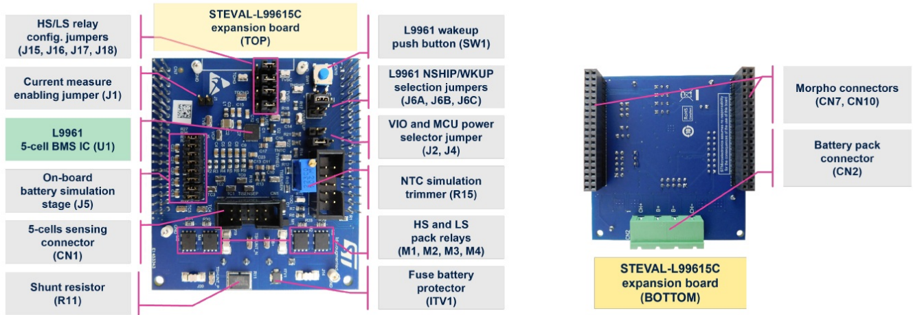
Figure 3. STEVAL-L99615C expansion board - top and bottom
