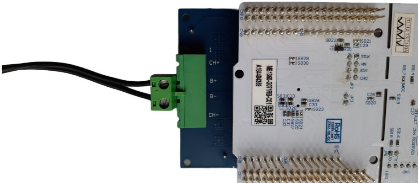
Figure 11. How to connect the power terminals to the battery
