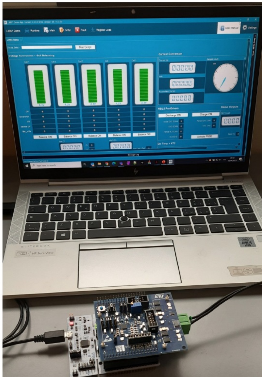
Figure 13. STEVAL-L99615C connected to a laptop (panoramic view)
