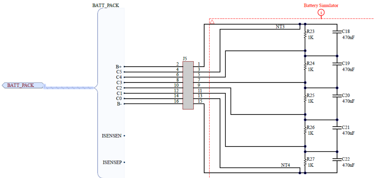
Figure 4. Power supply connector and battery simulator
