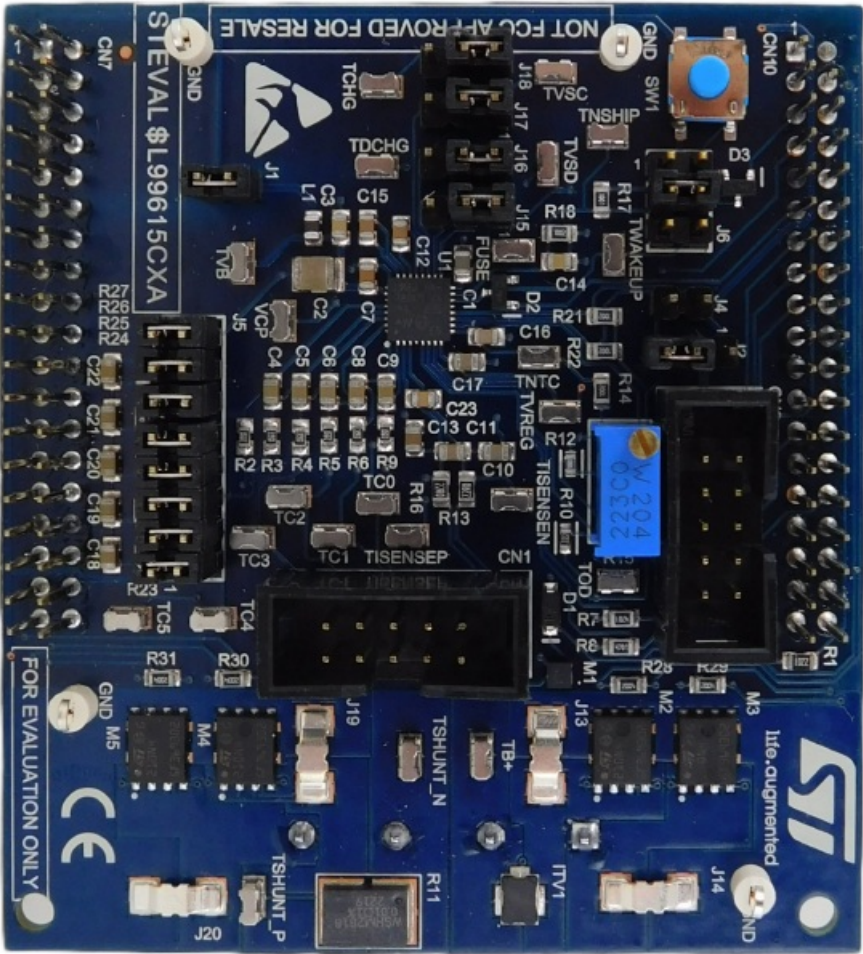
Figure 10. STEVAL-L99615C jumpers setting
