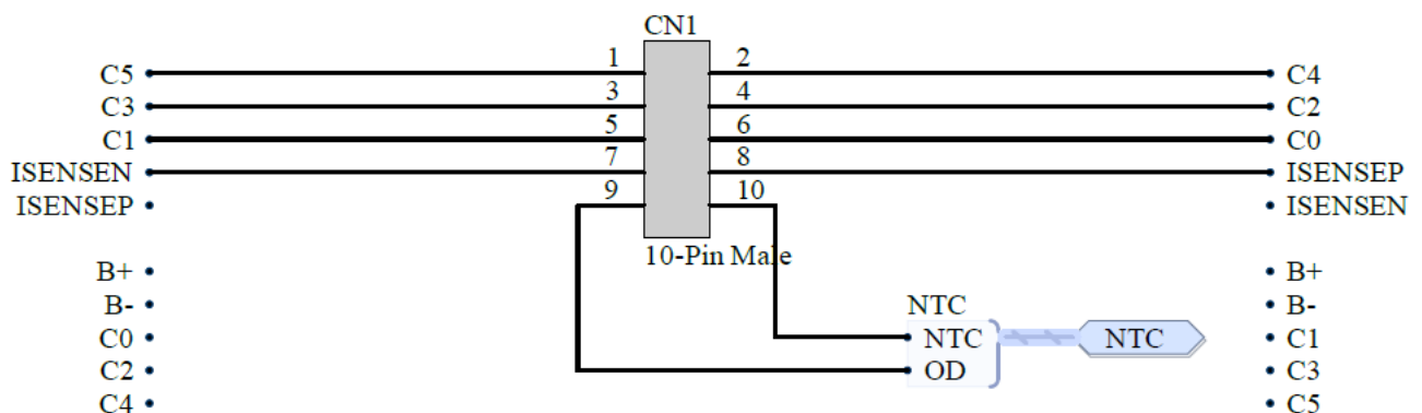
Figure 7. CN1 connector
