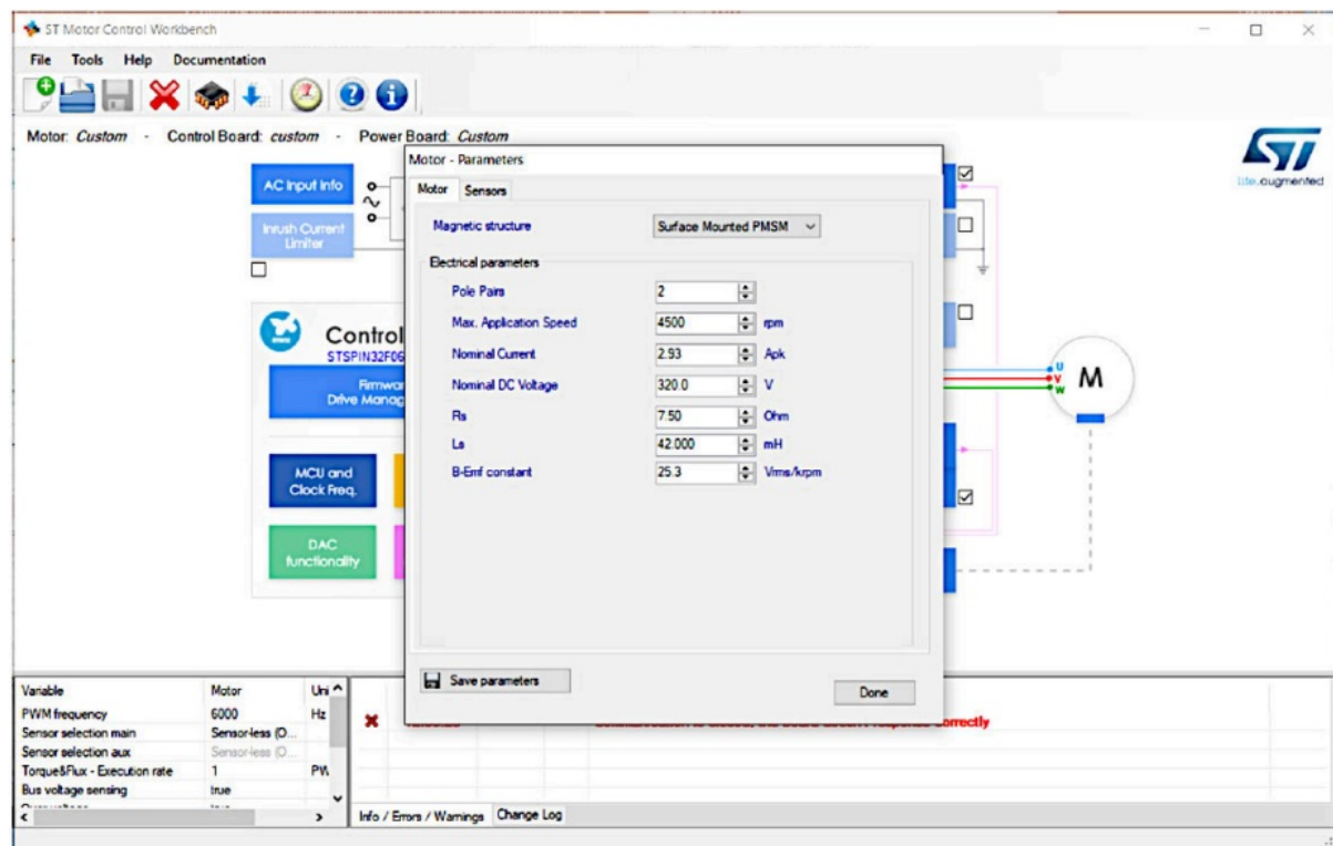
Figure 8. X-CUBE-MCSDK configuration example (2 of 2)
