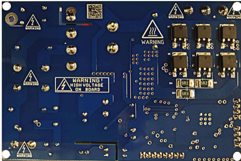
Figure 4. STEVAL-CTM011V1 – shunt configuration
