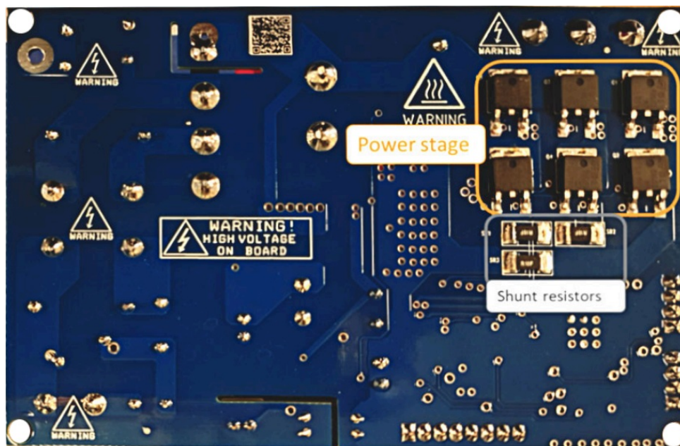
Figure 3. STEVAL-CTM011V1 main components (bottom view)
