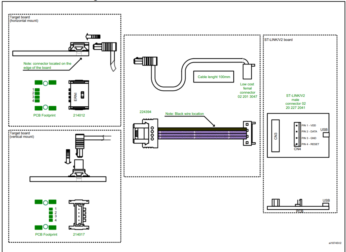
Figure 11. SWIM ST-LINK/V2 standard ERNI cable
