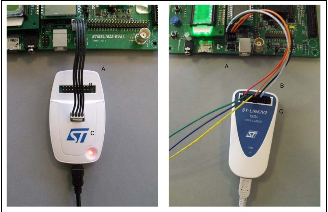
Figure 7. Low-cost connection
