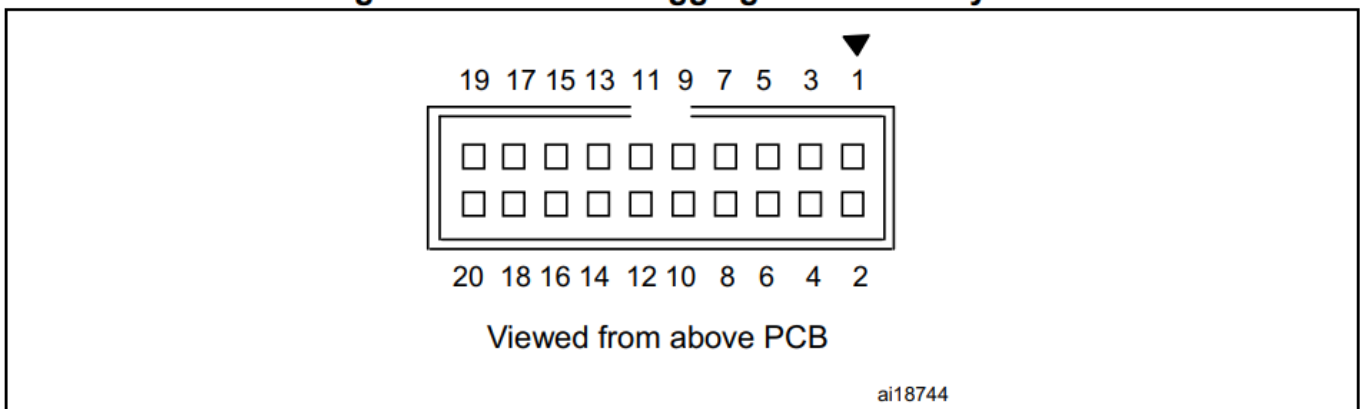
Figure 10. JTAG debugging flat ribbon layout
