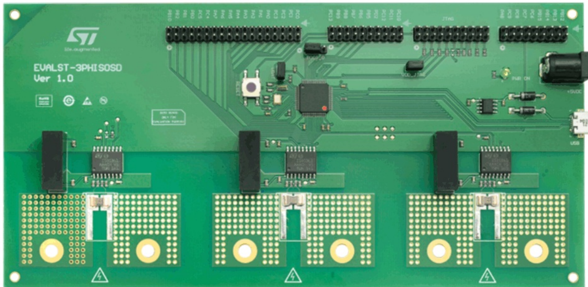
Figure 1. EVALST-3PHISOSD
