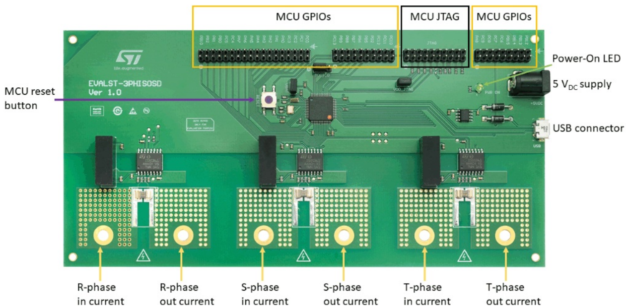
Figure 3. EVALST-3PHISOSD boards function description
