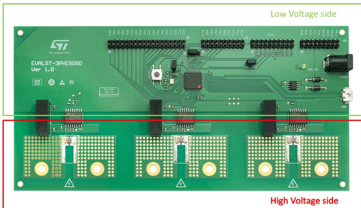
Figure 2. High and low voltage sides
