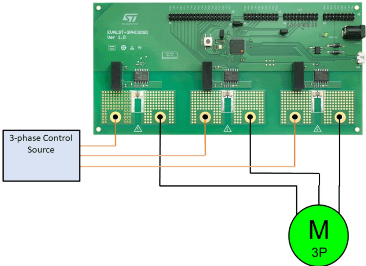
Figure 5. Electric connections (3-phase controlled motor)
