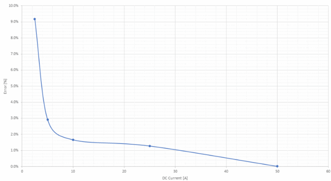
Figure 7. DC accuracy
