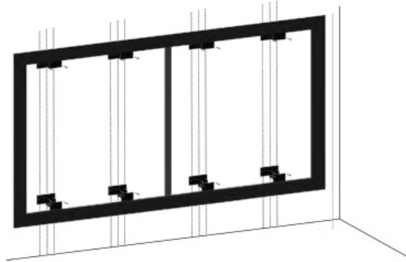
Figure 6: Mounting the frame with the Telescoping Mounts
