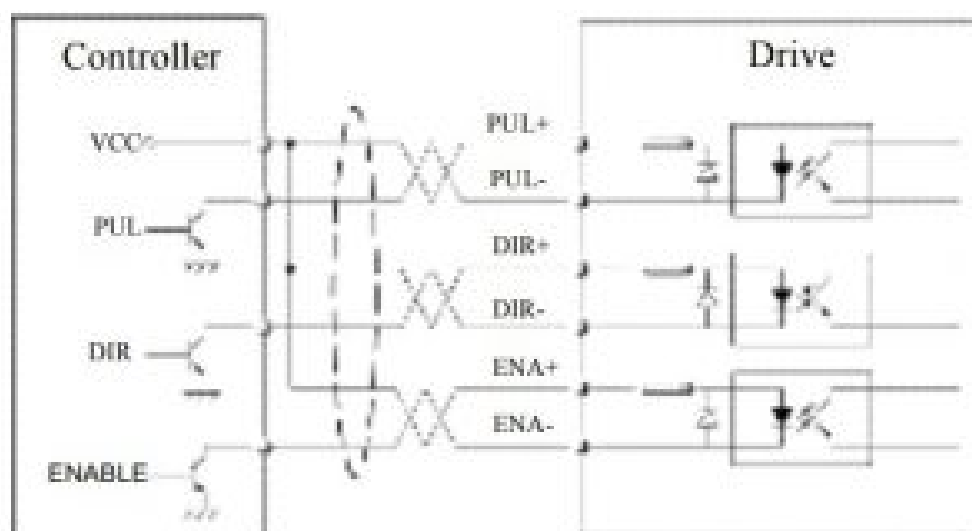
Figure 3: Connections to open-collector signal (common-anode)
