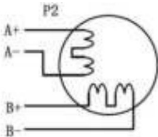
Figure 5: 4-lead Motor Connections
