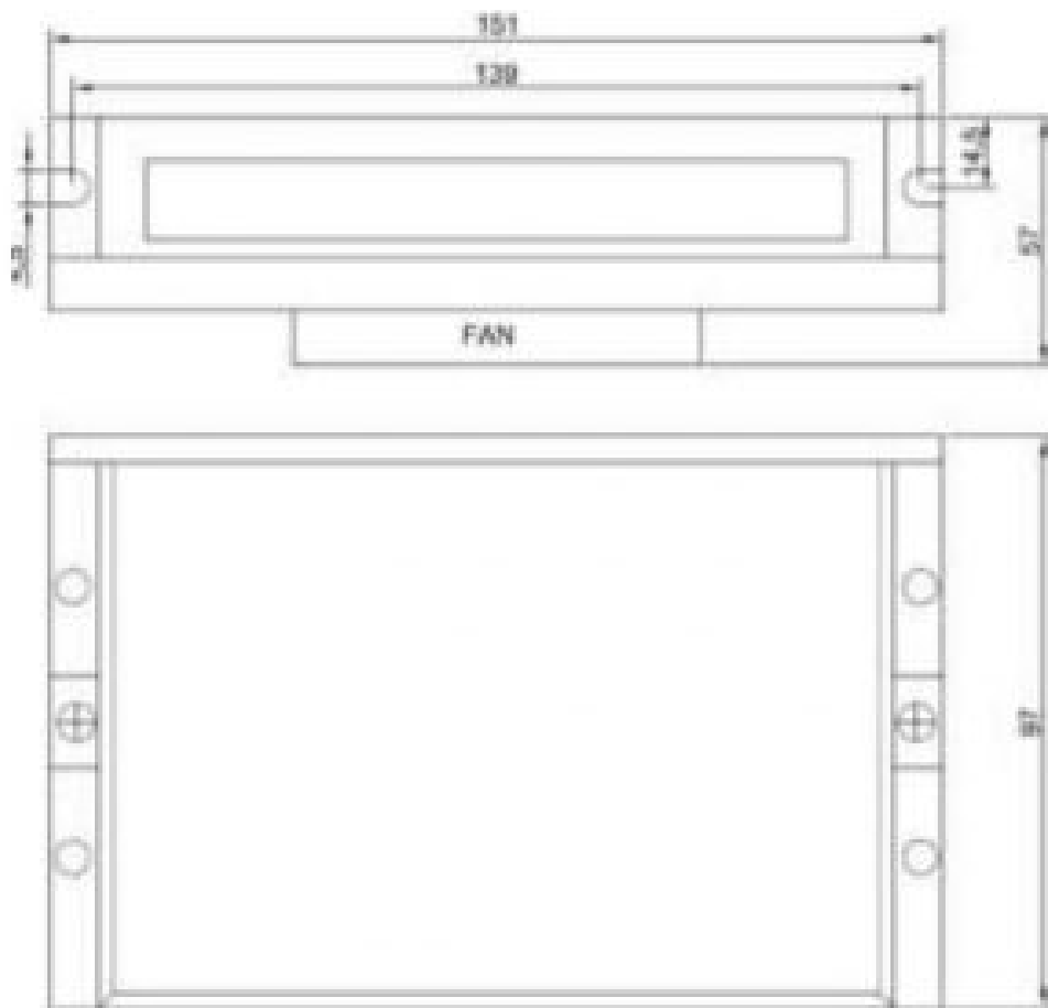
Figure 1: Mechanical specifications
