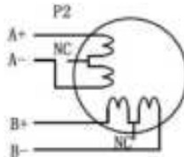
Figure 7: 6-lead motor full coil (higher torque) connections
