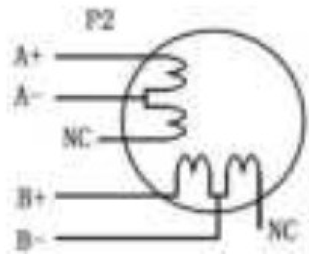
Figure 6: 6-lead motor half coil (higher speed) connections
