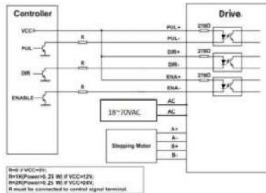
Figure 10: Typical connection
