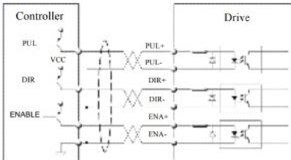
Figure 4: Connection to PNP signal (common-cathode)
