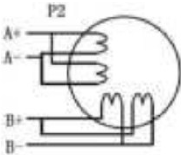
Figure 9: 8-lead motor parallel connections
