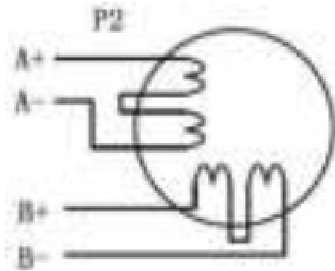
Figure 8: 8-lead motor series connections
