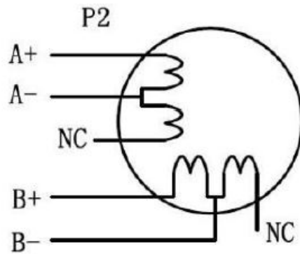
Figure 5: 6-lead motor half coil (higher speed) connections
