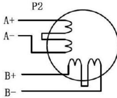
Figure 7: 8-lead motor series connections
