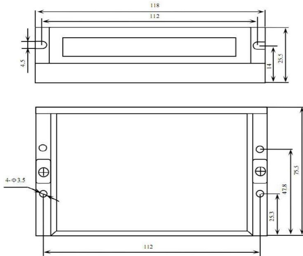
Figure 1: Mechanical specifications
