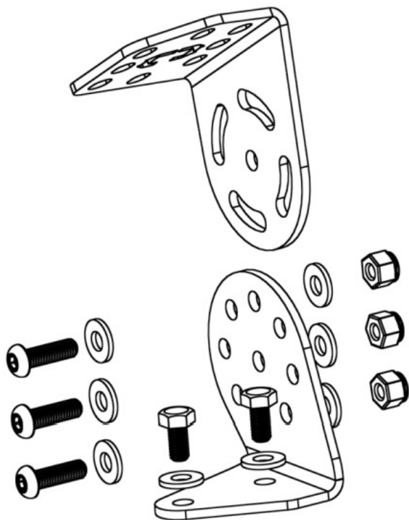
➞ SPACERAIL ANGLE MOUNT KIT Rail Kit and Hooks are sold separately
