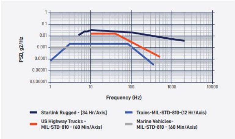
Figure 1: Comparison Across Common Use Vibration Test Profiles – Vertical Axis
