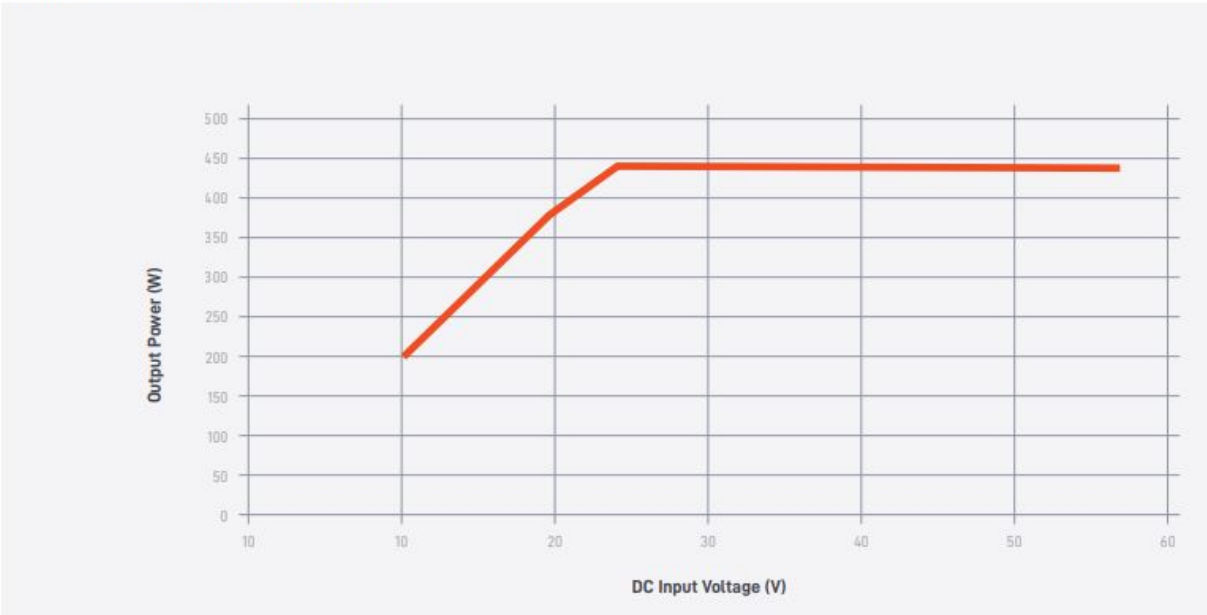
Figure 3: DC Input Voltage vs Output Power
