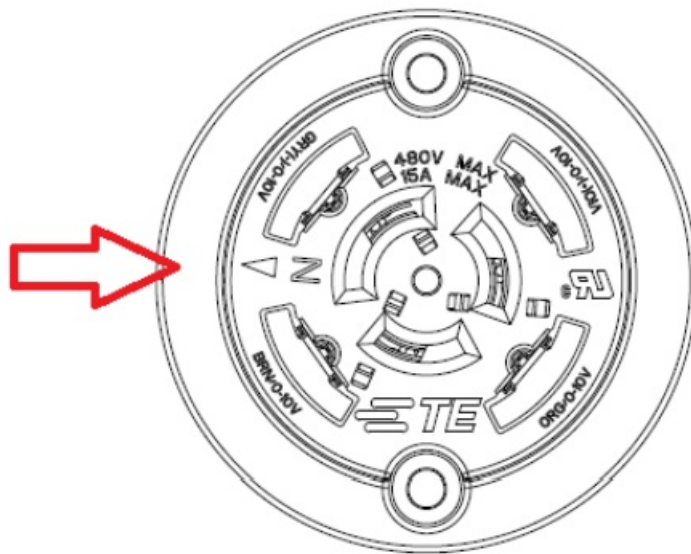
Figure 1 - Top view of the NEMA receptacle showing the North direction Warning:
