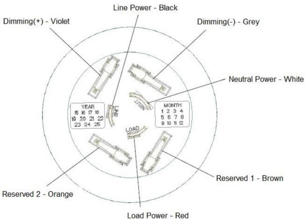
Figure 4 - LCU NEMA 7-Pin Contact Interface
