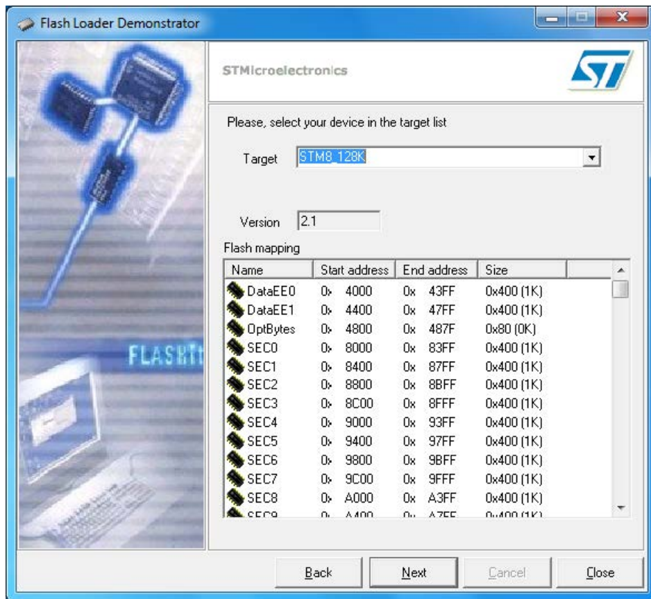
Figure 8. Device information page – STM8 example
