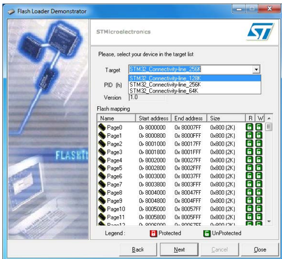
Figure 7. Device information page – STM32 example
