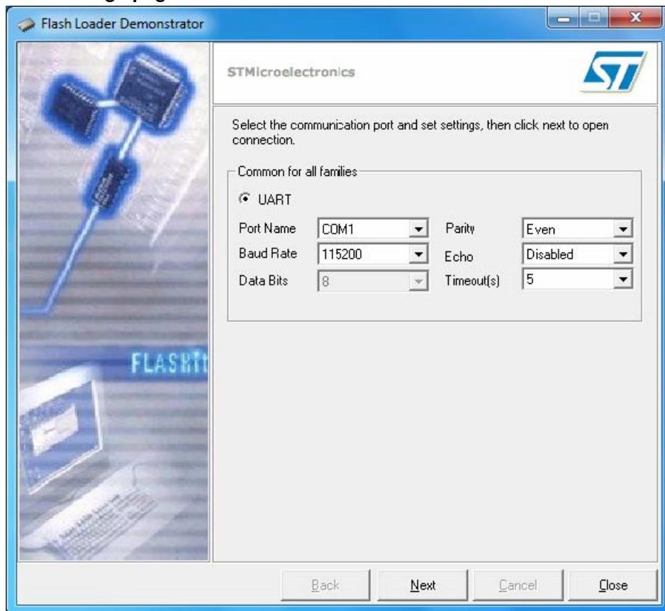
Figure 5. Connection settings page
