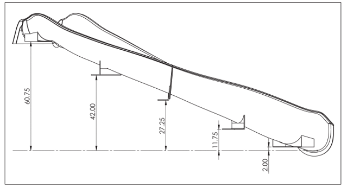
LEFT TURN WITHOUT SUPPORTS
