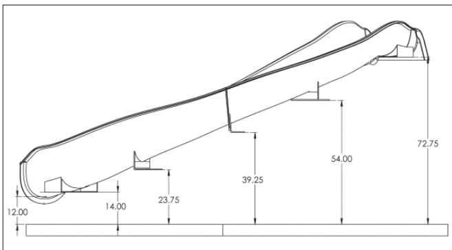
RIGHT TURN W/SUPPORTS
