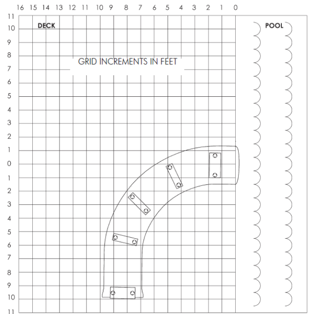
FIG. 8B – 15' GRS RIGHT TURN
