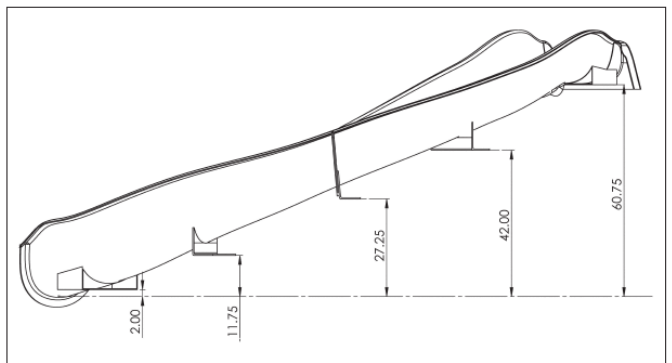
RIGHT TURN WITHOUT SUPPORTS
