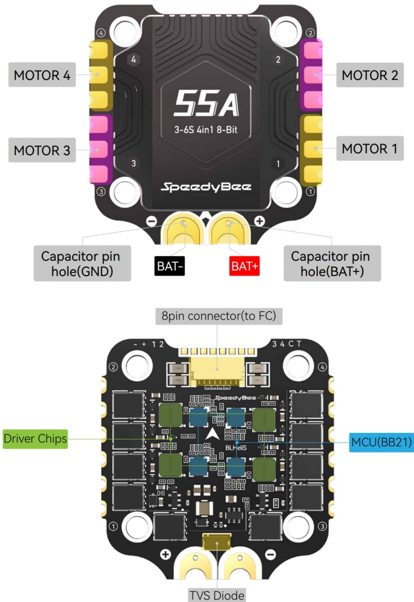
Connection with the flight controller & Motors
