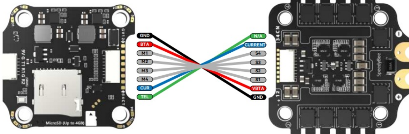
F405 V3 Flight Controller
